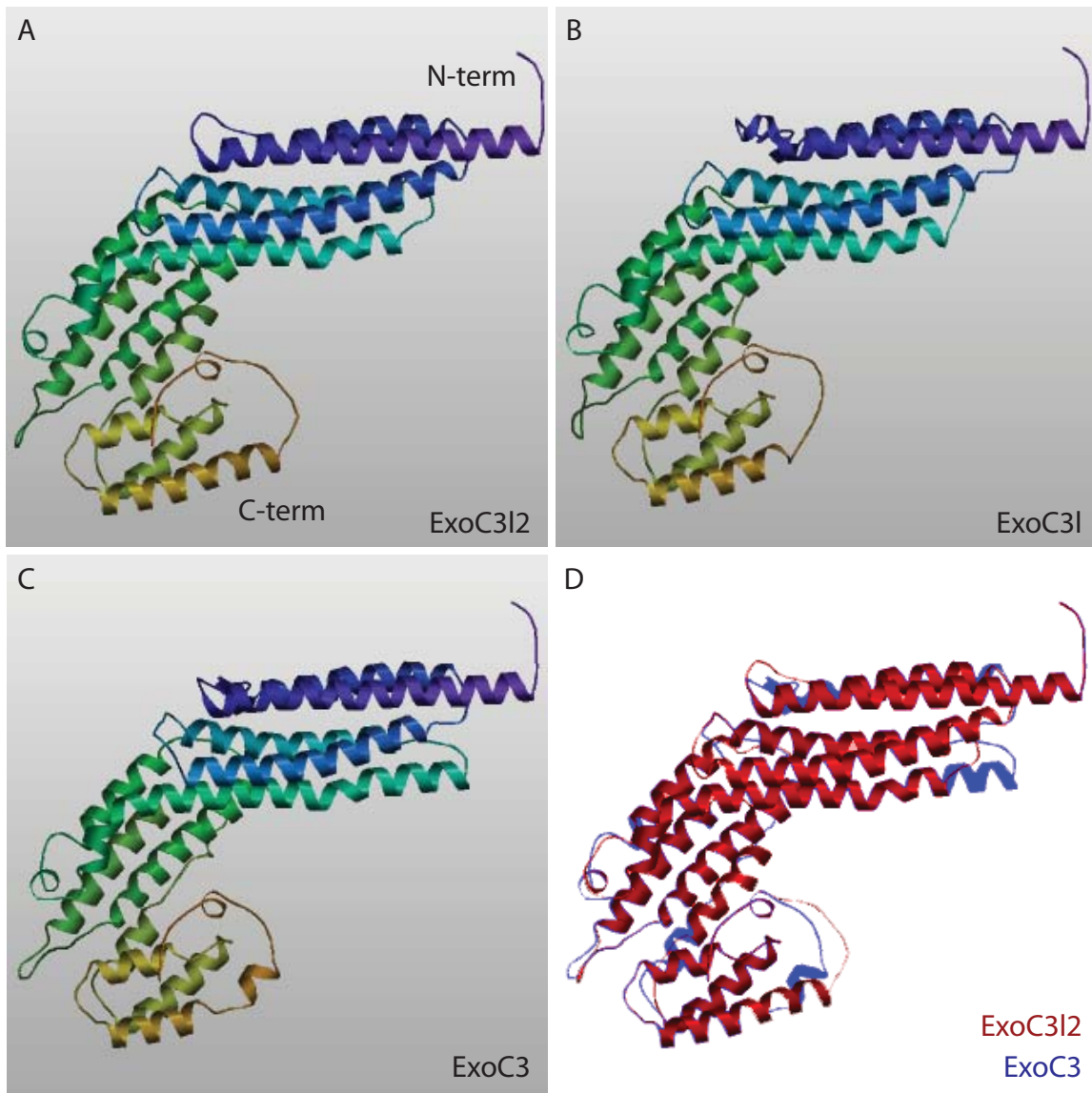
Supplemental Figure 1. Predictions of the tertiary structures of EXOC3L and EXOC3L2. (A-C) Predictions of the tertiary structures of EXOC3L2 (A) and EXOC3L (B) from the structure of the N-terminal domains of EXOC3 (ID:2FJI)(C) using SWISS-MODEL ( http://swissmodel.expasy.org ). (D) The models of EXOC3 (blue) and EXOC3L2 (red) superimposed.
