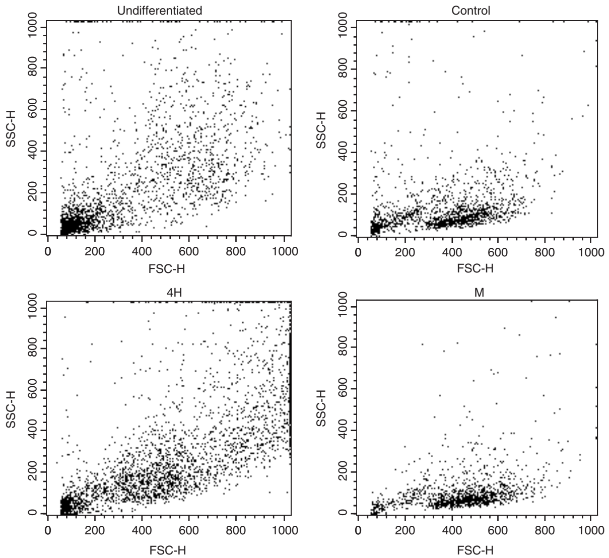
SUPPLEMENTARY FIG. 1. The forward scatter, given as dimensionless measures of mean fluorescence intensity, shows the relative size of the cell populations obtained in this study. The control treatment cells were the smallest, while the largest cells were obtained by treatment with BMP-4 + TGF- \beta 3.
