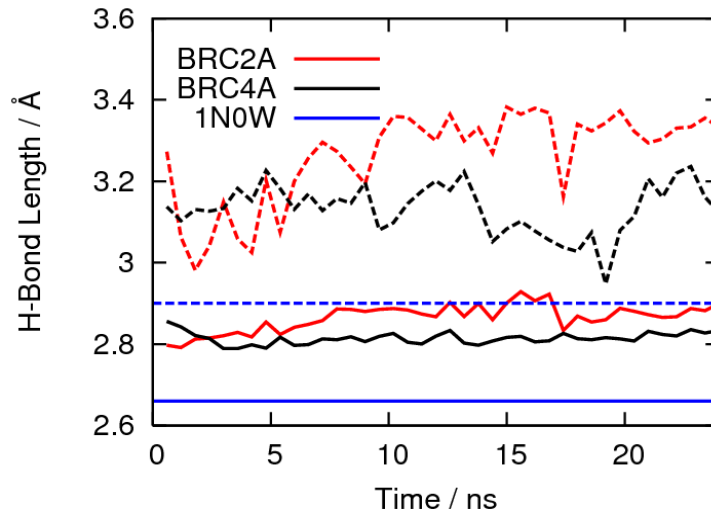
Figure S4. Block averages of two backbone inter-protein hydrogen bonds (solid and dashed lines) in simulations of the interaction between RAD51 and the BRC repeats, compared to the 1N0W crystal structure. The backbone hydrogen bonds are longer in the BRC2A interaction than in the BRC4A interaction, which may be a result of the different binding modes observed.
