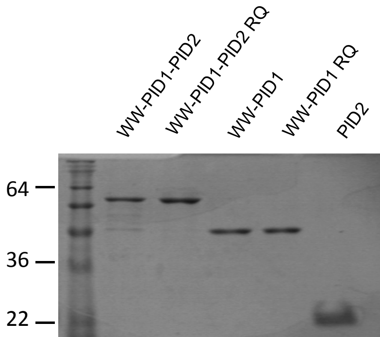
Figure S1. Fe65 WW-PID1-PID2 236-662, WW-PID1-PID2 R451Q 236-662, WW-PID1 236-512, WW-PID1 R451Q 236-512, and PID2 536-662 (1-2.5 \mu M) visualized on a 13% SDS-PAGE gel stained with Commassie.
