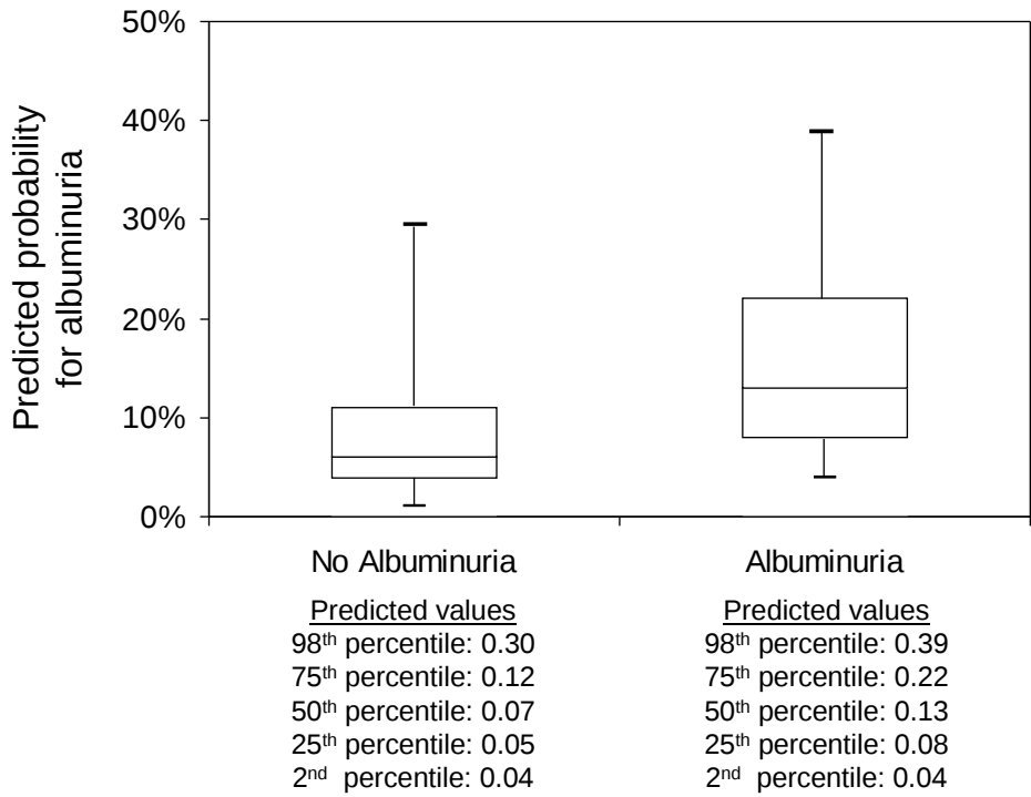
Supplemental Figure 1. Box plot of predicted probabilities for having albuminuria based on the self-assessment tool among individuals without and with albuminuria in the external validation data set (NHANES 1999-2004).
