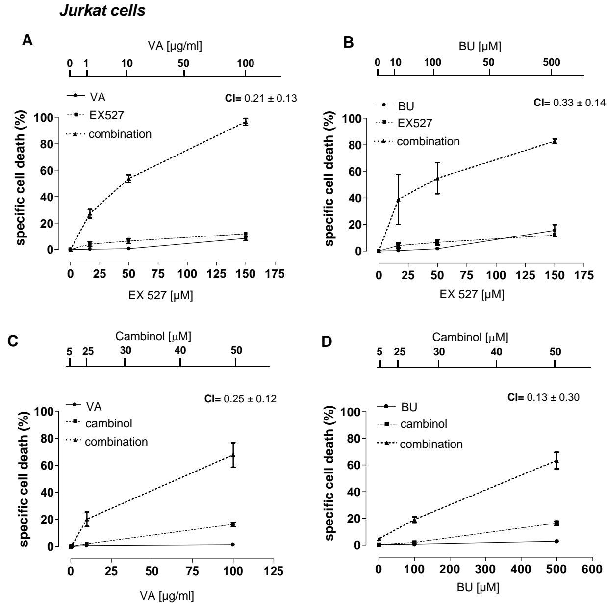
Figure S3. Sirtuin inhibitors and HDAC inhibitors synergistically kill Jurkat cells. A-D, Jurkat cells were incubated in 96-well plates with or without EX527, cambinol, BU, or VA at the indicated concentrations. Viability was assessed 48 h later by PI cell staining and flow cytometry. CI values refer to the highest drug concentrations used.
