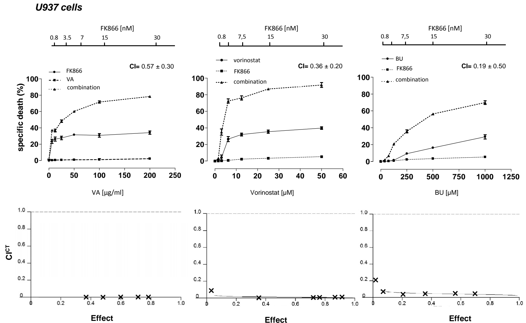
Figure S13. Synergistic interaction between FK866 and HDAC inhibitors in the AML cell line U937. U937 cells were incubated with or without FK866 at the indicated concentrations for 48 h. Thereafter, VA, vorinostat, or BU were added at the indicated concentrations. Viability was assessed 48 h later by PI cell staining and flow cytometry. CI values refer to the highest drug concentrations used. CI^{CT} s for each drug combination are shown in the lower insets.
