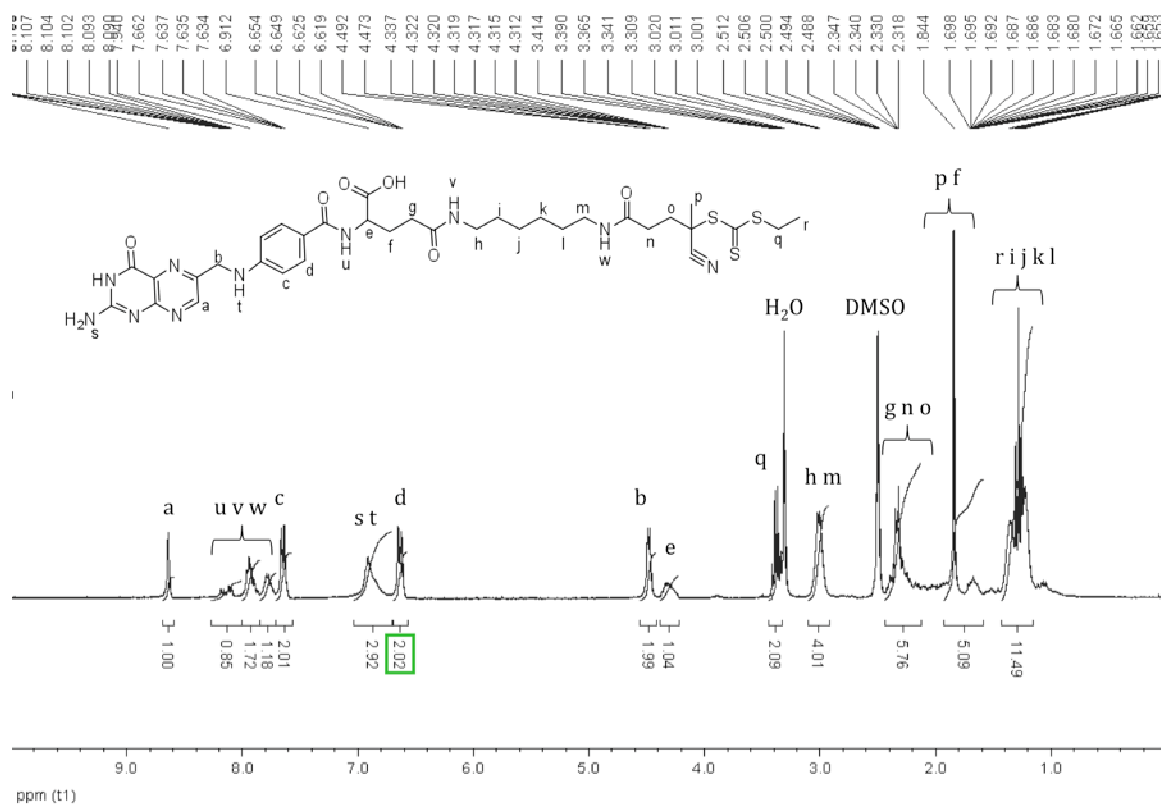
Figure S1. 1 H-NMR spectra of the folate-functionalized CTA.
