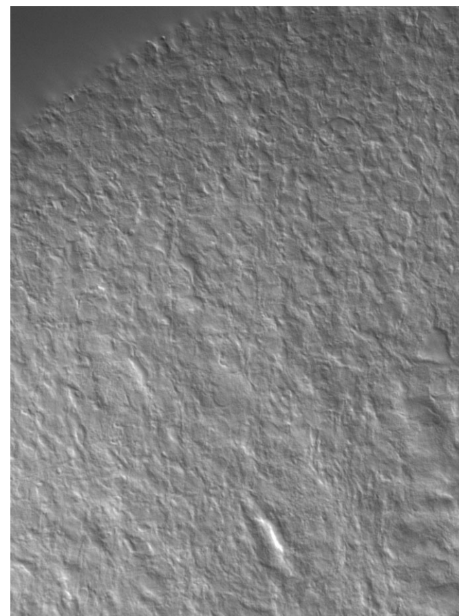
dlx RNAi
