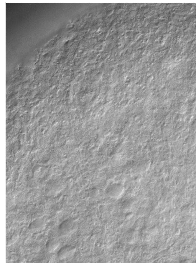
six1/2 RNAi
