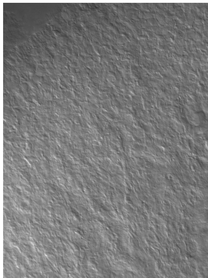
sp6-9 RNAi
