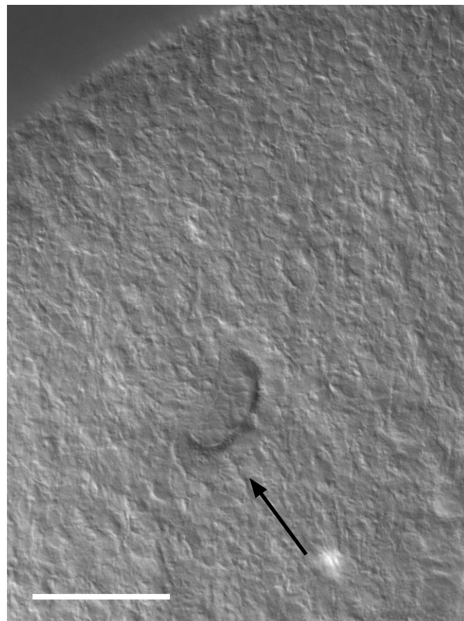
Control RNAi
