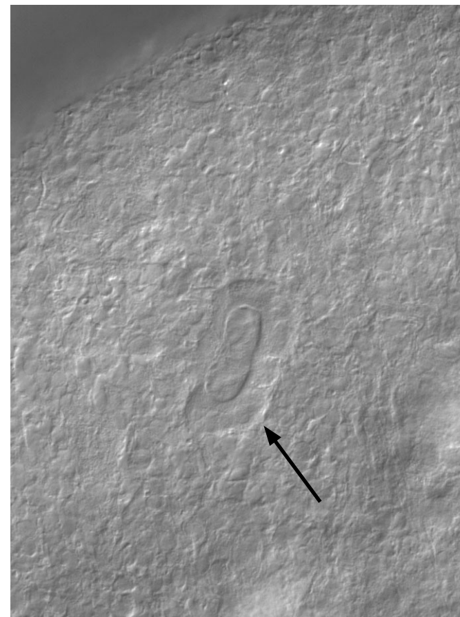
tyrosinase RNAi
