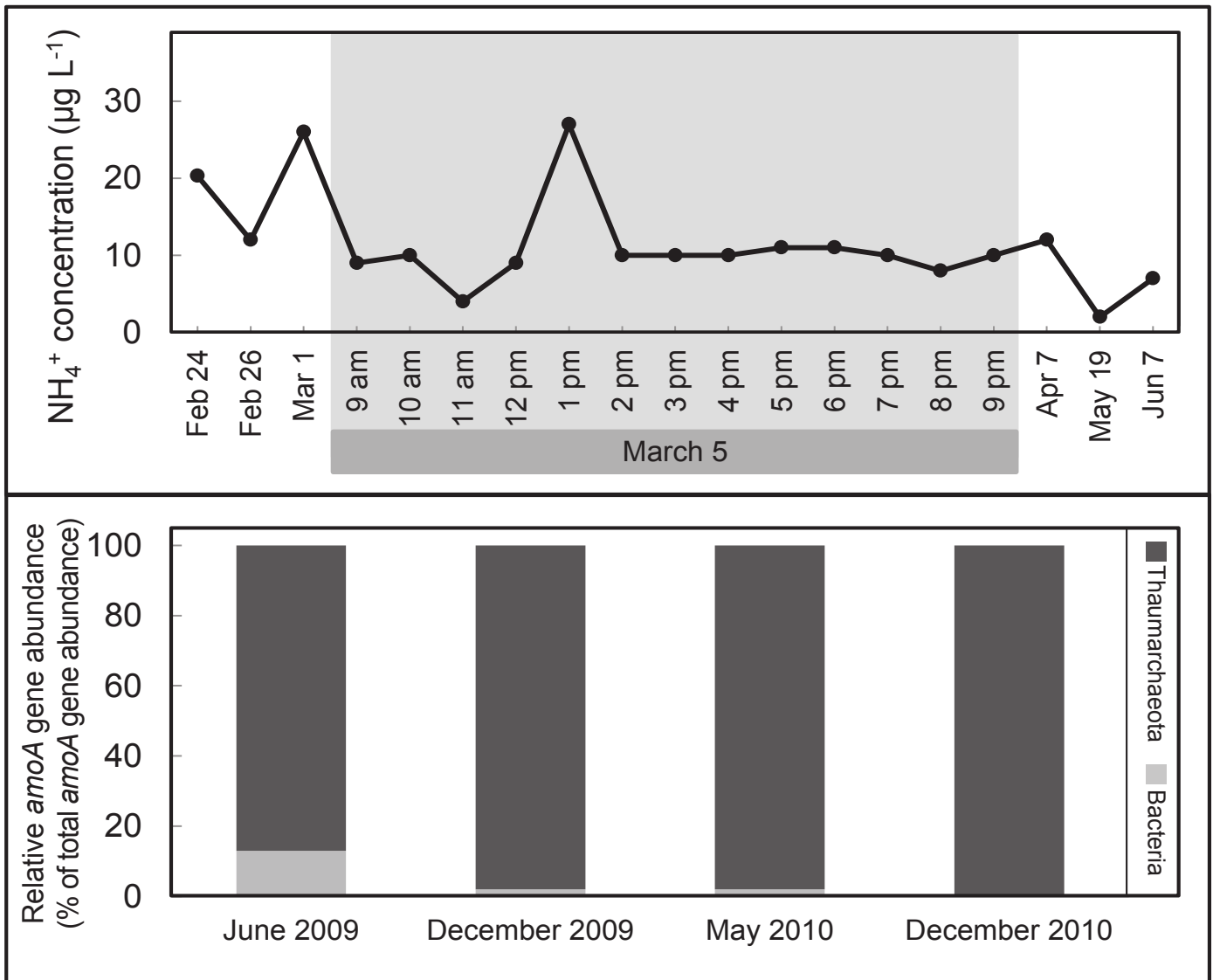
Figure S1. Aquarium FW27 temporal patterns. Ammonium concentrations (A) are shown over several months (during 2010), and hourly over a 12 hour period. Proportions of AOA/AOB in the FW27 sponge filter DNA extract are shown from four time points over the course of 2 years.
