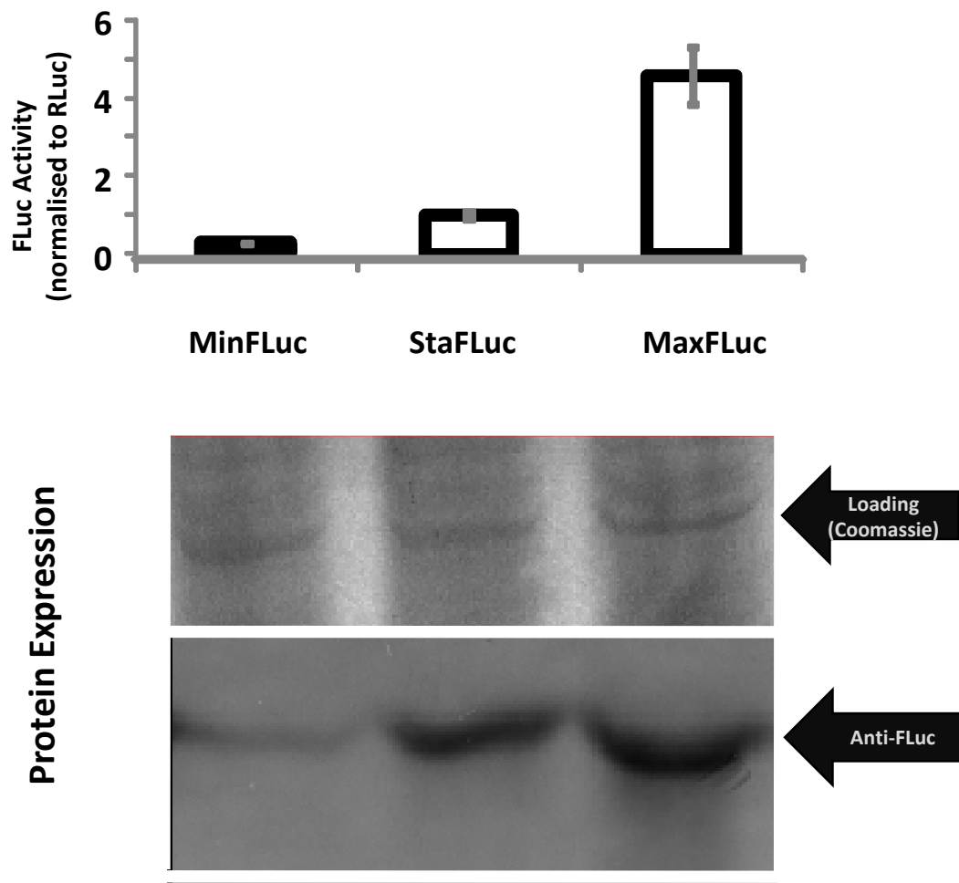
Supplemental Figure 1. Gene expression levels from different Firefly luciferase (Fluc) encoding sequences in yeast strain BY4741 \Delta dom34 . Top, activity levels as measured by dual-luciferase assay. Bottom, actual protein expression levels as determined in western blots. Both assays indicate a 5-fold change in expression levels between MinFLuc and StaFLuc, and between StaFLuc and MaxFLuc.
