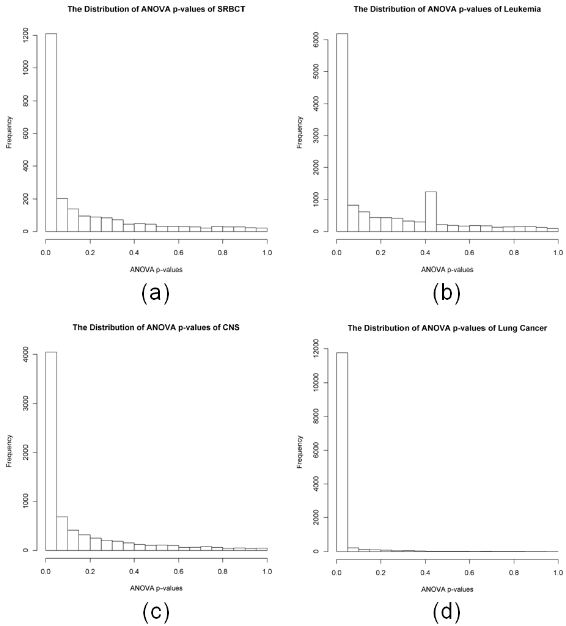
Figure S5. The distributions of ANOVA p-values for four datasets.
