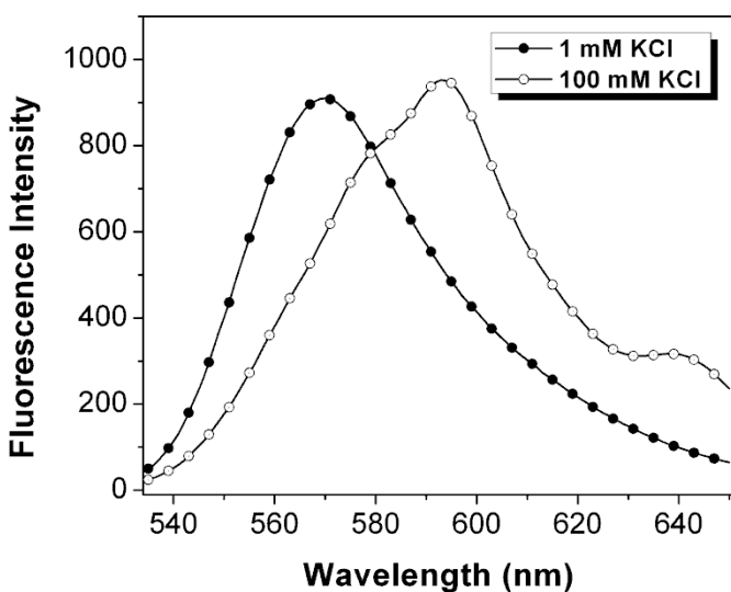
Figure S1. Effect of KCl on the fluorescence emission spectrum of 1.0 μM β-Me-DiSC 1 (3) in the presence 0.5 μM Myc19 DNA quadruplex. Samples were excited at 520 nm.
