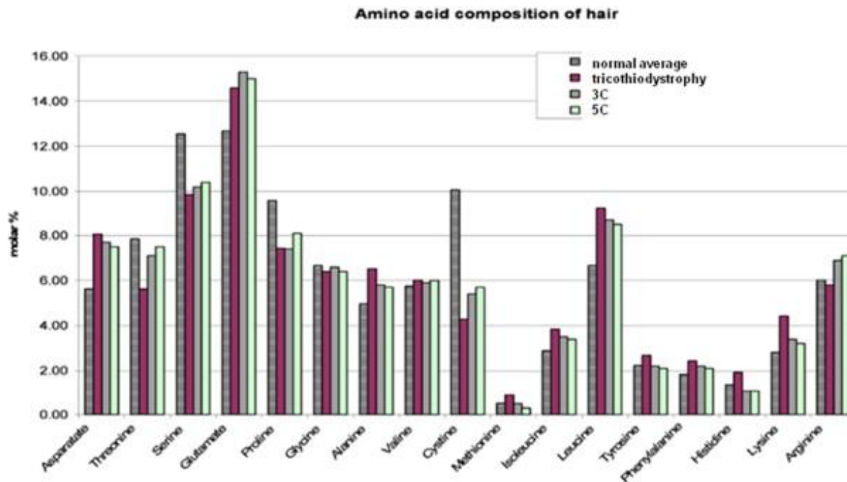
Supplementary Figure 1 The amino acid composition of hair from 2 of the patients with THES shows a remarkable similarity to the amino acid composition of hair from children with trichothiodystrophy.
