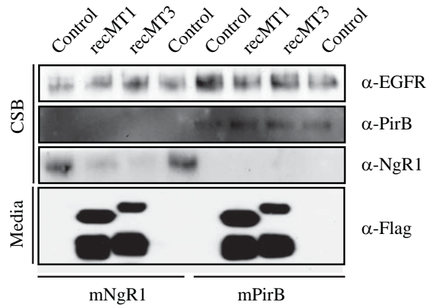
Fig S2. Recombinant MT-MMPs 1 and 3 do not cleave PirB. Western blot analysis of cell surface biotinylated proteins and conditioned media from COS-7 cells transfected with mNgR1 or mPirB and treated with 1 \mu M recombinant MT1-MMP or MT3-MMP for 6 hours. MT1-MMP and MT3-MMP reduce cell surface levels of Ngr1 but not PirB. Endogenous EGFR (epidermal growth factor receptor) is blotted as a control for the cell surface biotinylation. The conditioned media is probed with an anti-FLAG antibody to detect recombinant MMPs.
