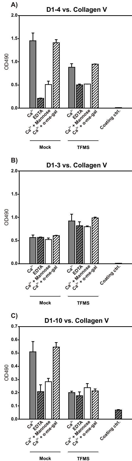
Figure S1. Binding of recombinant uPARAP variants to deglycosylated collagen type V. Binding of recombinant uPARAP variants to mock treated and deglycosylated collagen was performed and represented as described in the legend to Fig. 4, except that the treated collagen was type V.
