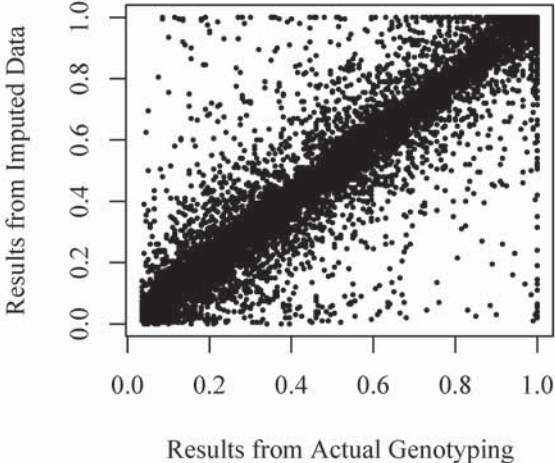
b) Estimates of LD Between Genotyped SNP and Untyped SNP
