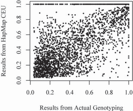
a) Estimates of LD Between Two Ungenotyped SNPs
