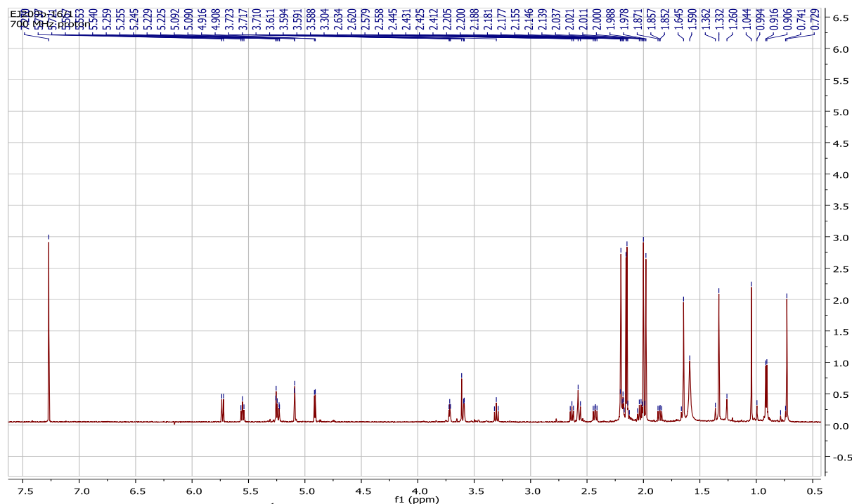
^1\text{H} NMR spectrum of taccalonolide AA
