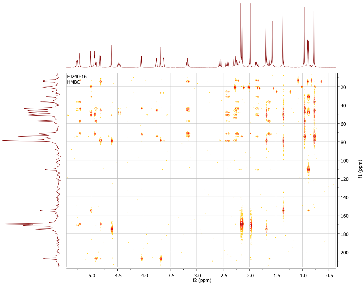
HMBC spectrum of taccalonolide AB
