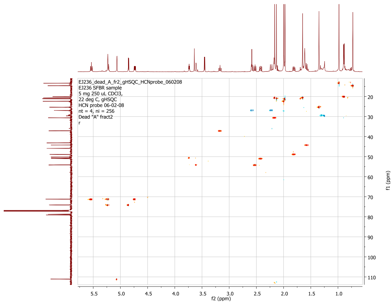
HSQC spectrum of taccalonolide Z
