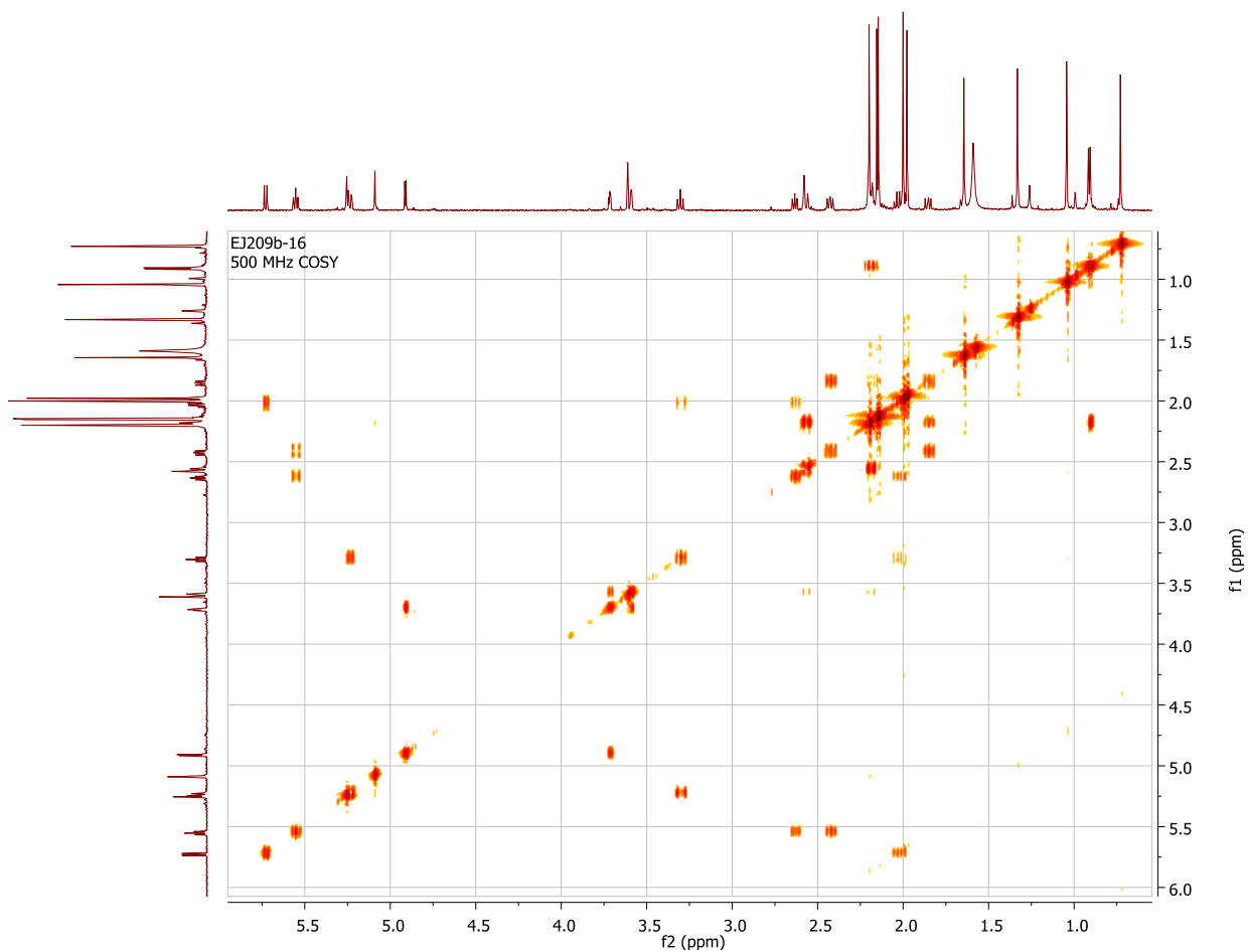
COSY spectrum of taccalonolide AA
