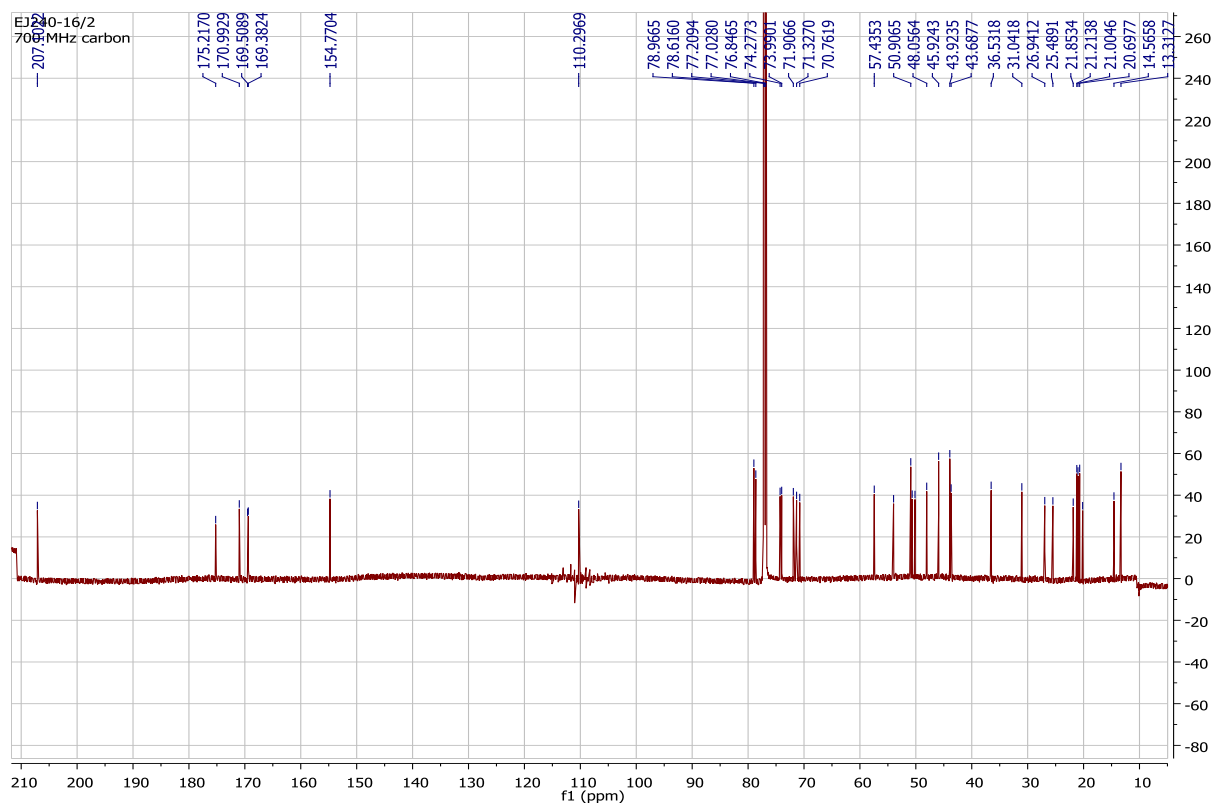
13 C NMR spectrum of taccalonolide AB
