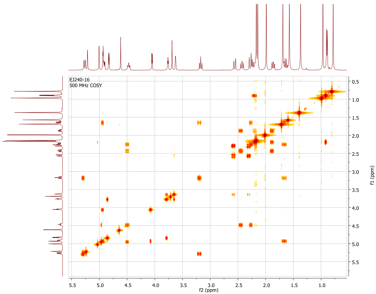
COSY spectrum of taccalonolide AB
