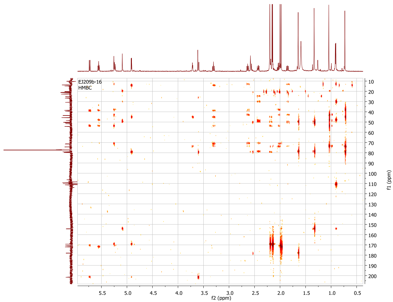
HMBC spectrum of taccalonolide AA
