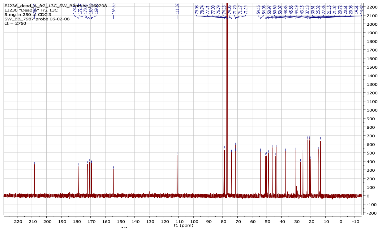
13 C NMR spectrum of taccalonolide Z
