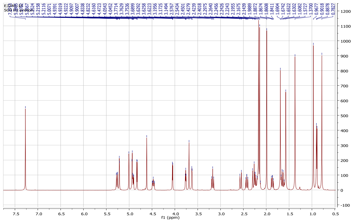
1 H NMR spectrum of taccalonolide AB
