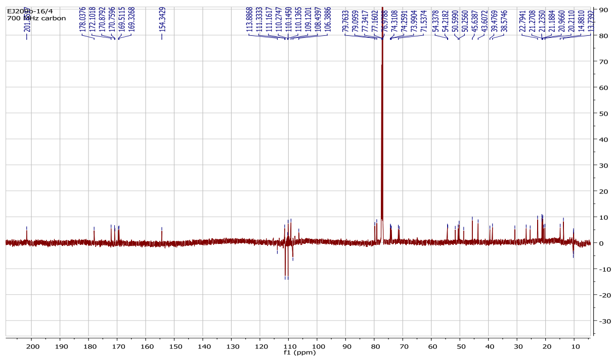
^{13}\text{C} NMR spectrum of taccalonolide AA
