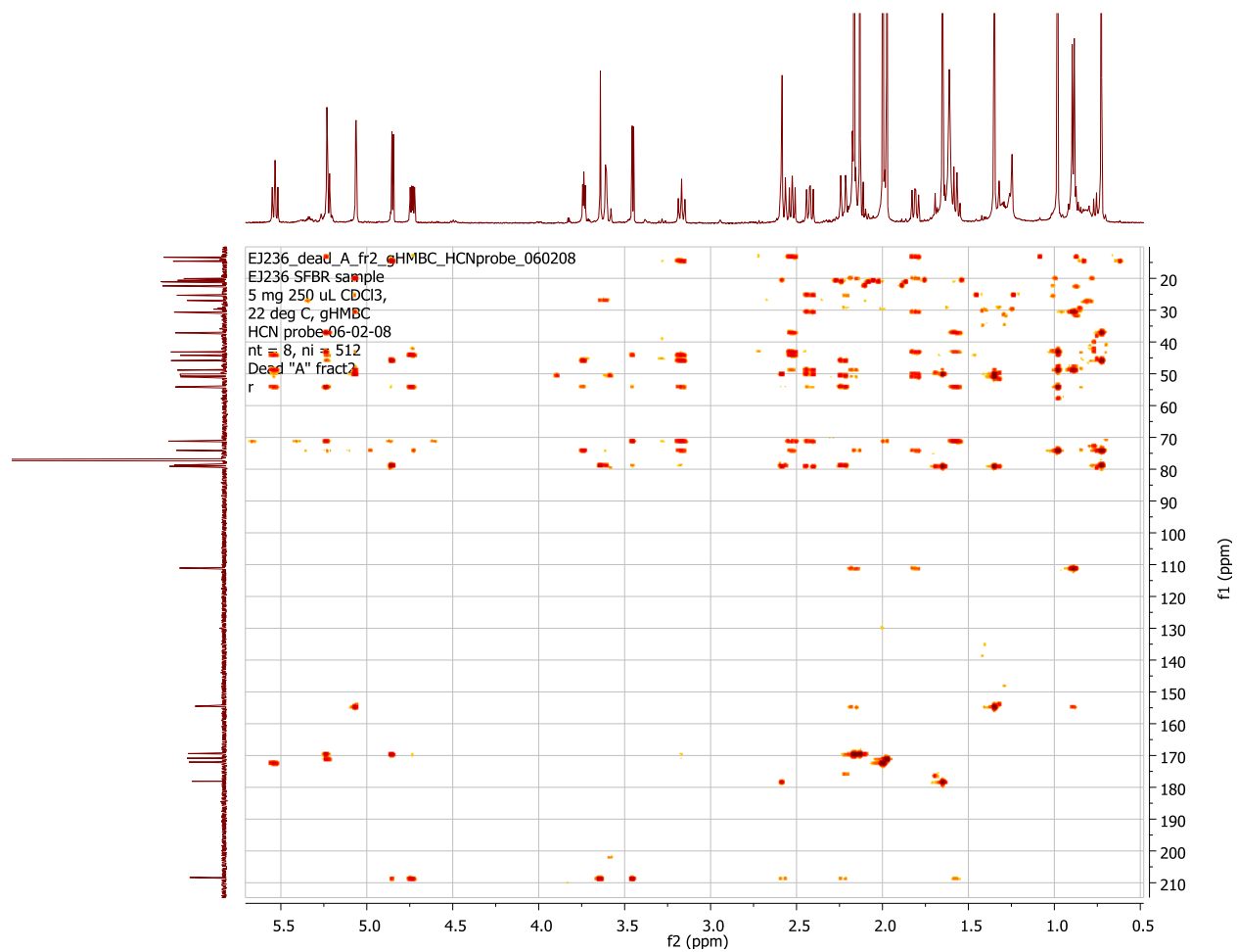
HMBC spectrum of taccalonolide Z
