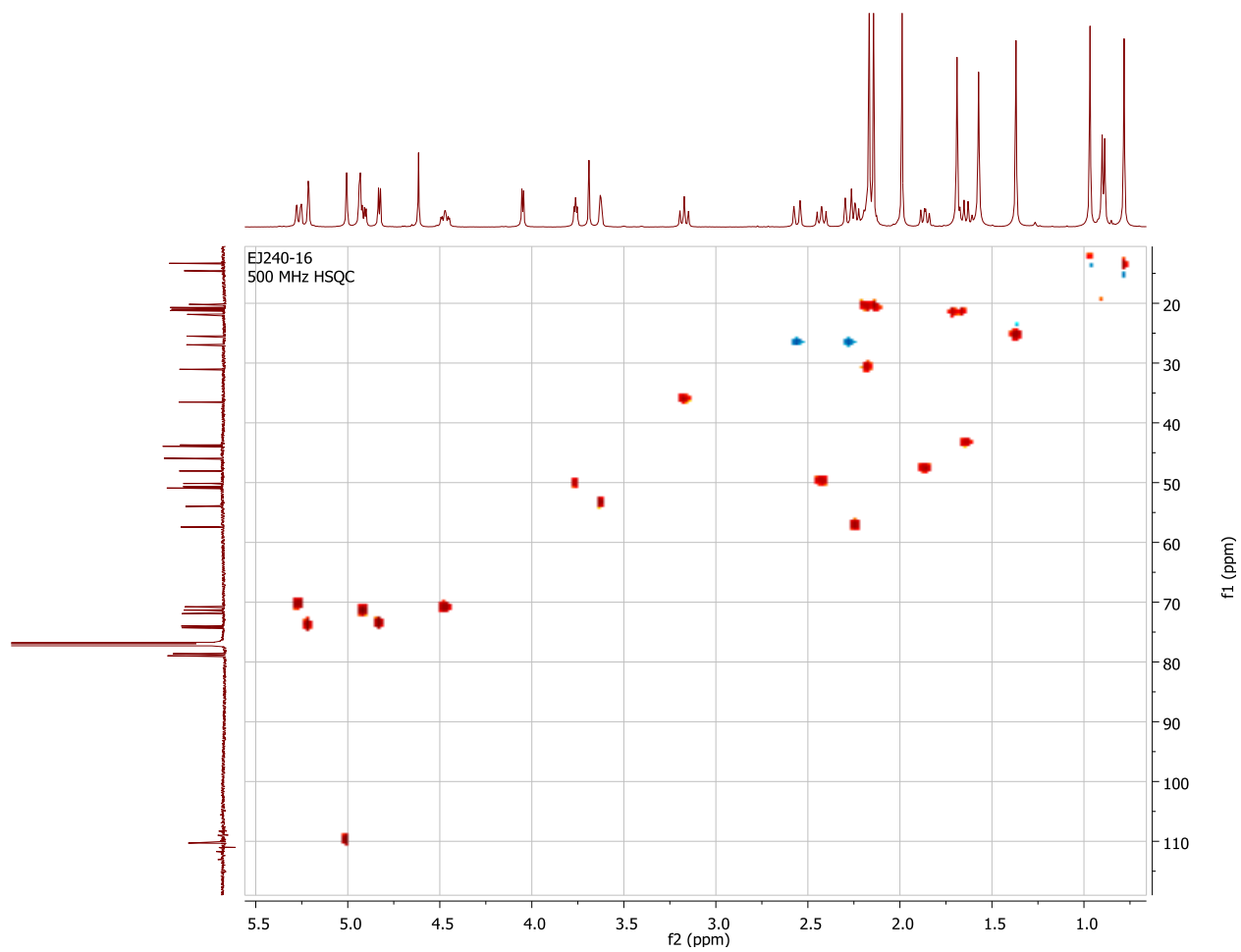
HSQC spectrum of taccalonolide AB
