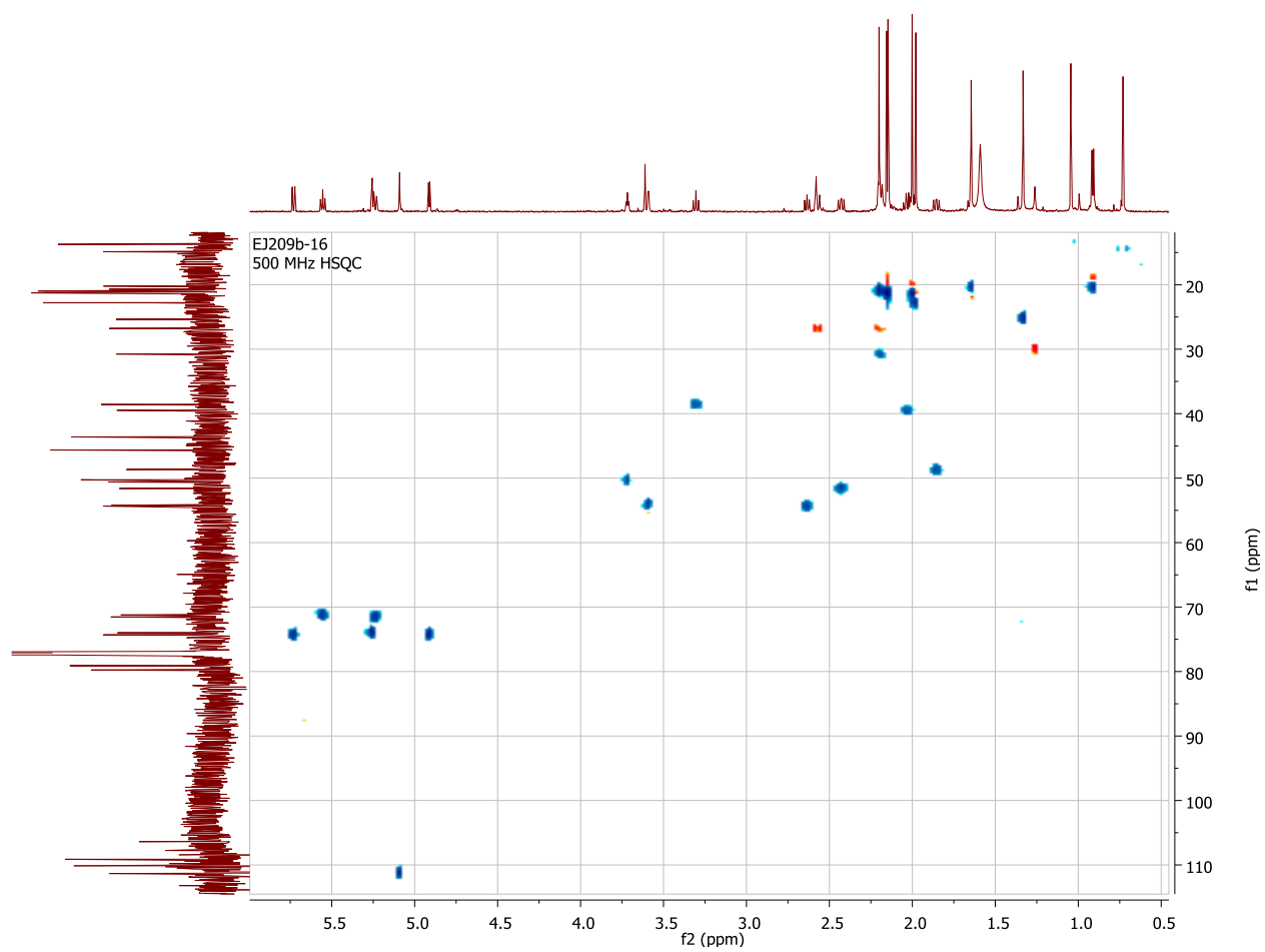
HSQC spectrum of taccalonolide AA
