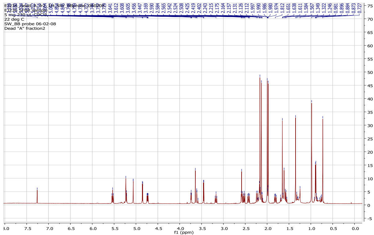
1 H NMR spectrum of taccalonolide Z
