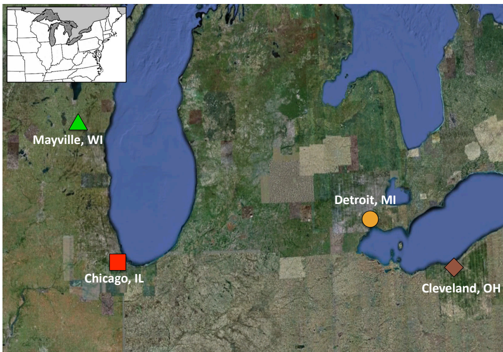
FIG S1. Map of the locations from which aerosol samples were collected over approximately a five week time span during summer and winter seasons, 2007. Symbols indicate the four cities surveyed in this study ( \blacktriangle = Mayville, \blacksquare = Chicago, IL, \bullet = Detroit, MI, and \blacklozenge = Cleveland, OH). Inset is an expanded view of the Midwest region, U.S.A. Maps reprinted from Google Earth.
