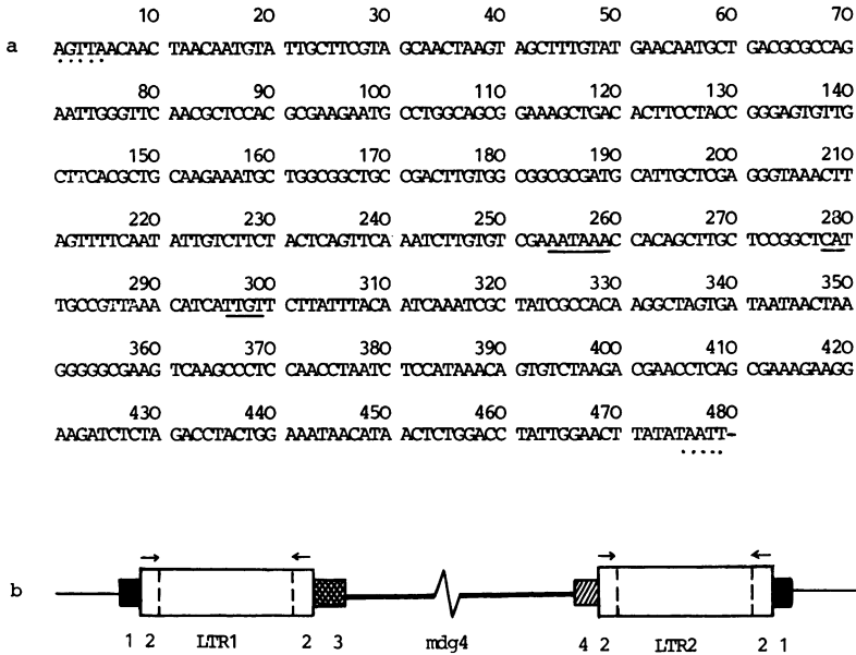
Fig. 5. Nucleotide sequences of mdg4 LTRs present in Dm111 and Dm112 clones (a) and schematic presentation of mdg4 LTRs and flanking sequences (b). 1 - duplication of host DNA; (2) mismatched inverted repeat; 3 - region of partial homology to tRNA Lys ; 4 - purine-rich region.
