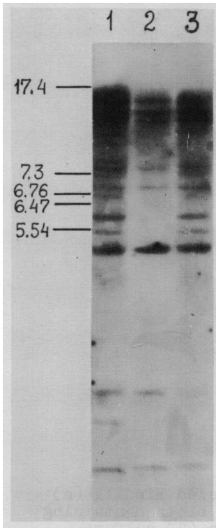
Fig. 3. Hybridization of Dm111 ^{32} P-labeled XhoI fragment to Southern blot containing BamHI restricted D. melanogaster DNA isolated from (1) embryos, (2) larval salivary glands, (3) adult Oregon RC flies. The BamHI restricted \lambda DNA was used as size markers.
