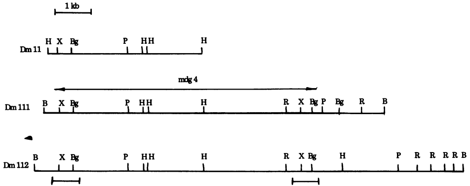
Fig. 1. Restriction maps of cloned fragments of D. melanogaster DNA containing mdg4 .
