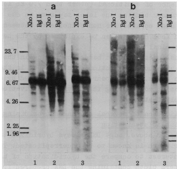
Fig. 2. Hybridization of Dm111 ^{32}\text{P} -labeled HindIII-EcoRI (1), HindIII (2), and XhoI (3) fragments to Southern blots containing restricted D. melanogaster DNA isolated from culture cells (a) and from Oregon RC flies (b). The amount of Oregon RC DNA was 2.5 times greater than that in DNA from culture cells. The HindIII restricted \lambda DNA was used as size markers.
