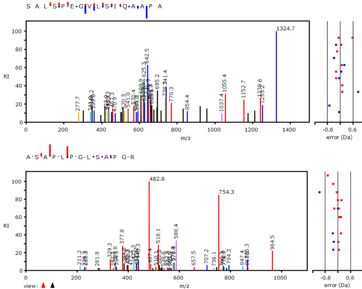
Supplementary Figure 2. Collision-induced dissociation spectra from an LTQ orbitrap that have led to the identification of Hsp20 in an immunoprecipitate from a P myometrial strip lysates. y-ions are depicted in red, b-ions in blue and unassigned ions in red. The sequence of the two peptides ^{134}\text{SALSPEGVLSIQAAAPA}^{146} and ^{15}\text{ASAPLPGLSAPGR}^{27} are on the top right of each spectrum annotated with the detected y- and b-ions with the same colour coding as in the spectra. The graphs on the right of the spectra illustrate the mass errors.
