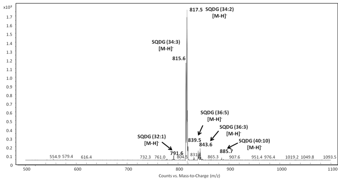
Figure S3: Precursor ions scan for SQDG in C. velia
