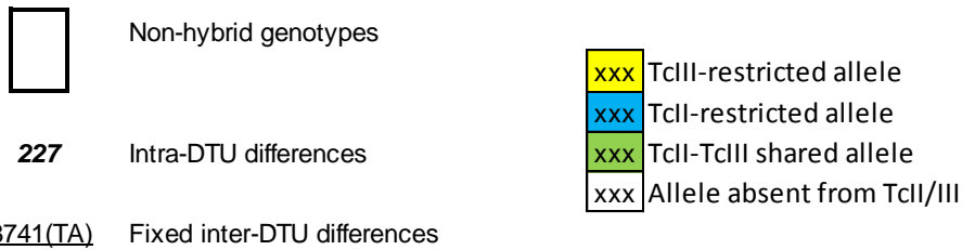
Supplementary Figure S1. Inferred patterns of allelic inheritance in hybrid multilocus genotypes
