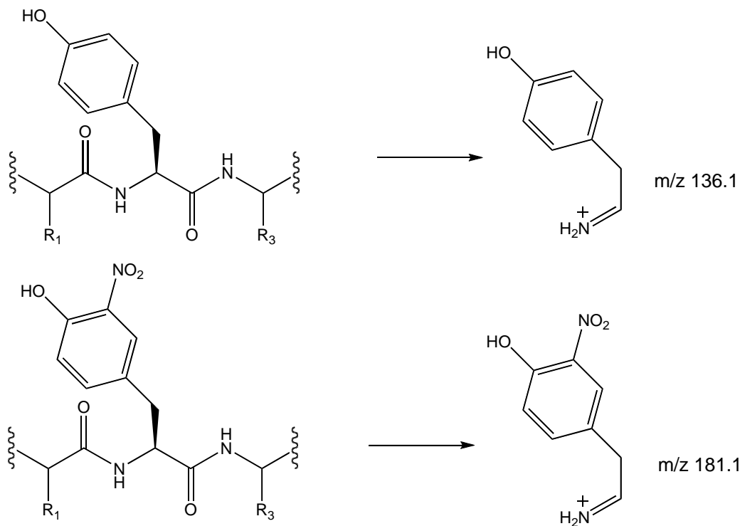
Supplementary Figure S4. Tyrosine and 3-nitro-tyrosine in a peptide chain and the corresponding immonium ion products after gas-phase fragmentation
