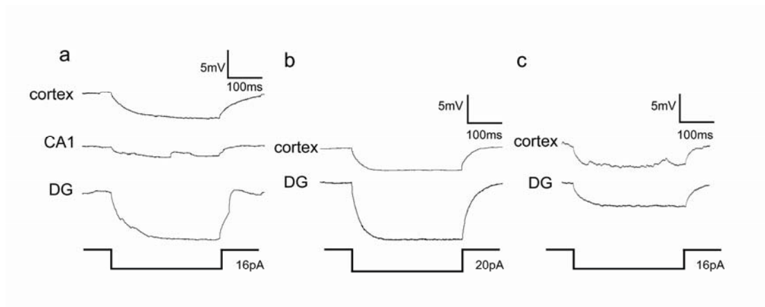
Figure S6 Comparison of voltage changes evoked by current pulses. (a) Adult mouse (C57/B6L, 8 weeks, male) neurons recorded from the indicated brain regions. Experiments are performed by Lab A. (b) Adult mouse neurons recorded from the indicated brain regions. Experiments are performed by Lab B using a different patch clamp and recording apparatus. (c) Adult rat (SD rat, 8 weeks, male) neurons recorded by Lab A from the indicated brain regions.
