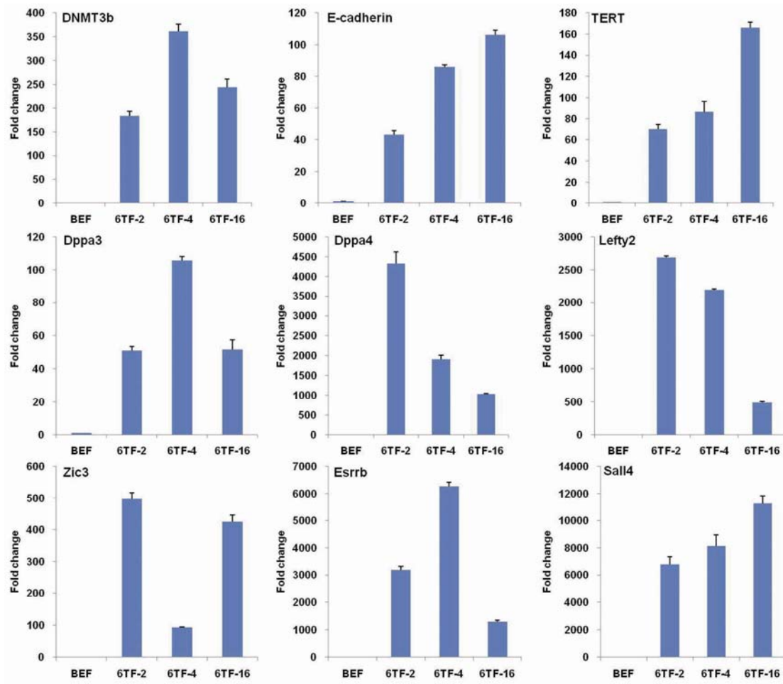
Supplementary information, Figure S3 Other pluripotent gene expression levels of biPS cells.
