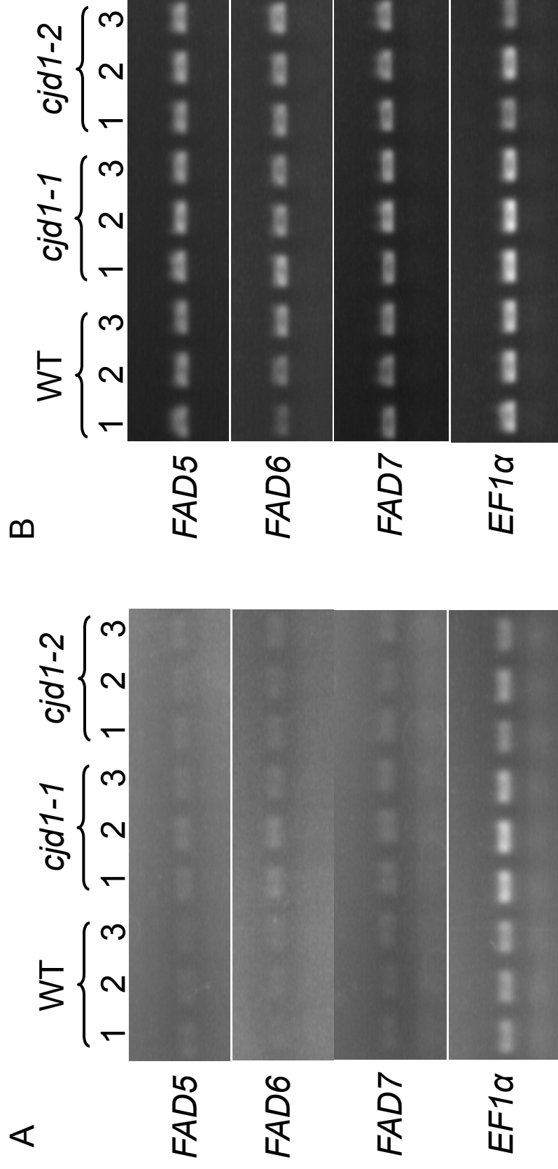
Figure S2. Steady-state transcript abundance of FAD5 , FAD6 , FAD7 and EF1 \alpha in wild-type (WT), cjd1-1 and cjd1-2 plants. A, 25 and B, 30 cycles into the RT-PCR analysis. Three biological replicates (1,2,3) were tested.
