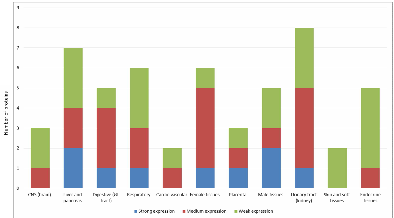
Supporting Figure 1. Annotation of oxidized proteins according to their tissue of origin. Differentially oxidized proteins in the diabetic Zucker rat plasma relative to their lean controls were searched in the protein atlas database and their degree of expression as indicated by the database (low, medium, strong) was plotted against tissue of origin.
