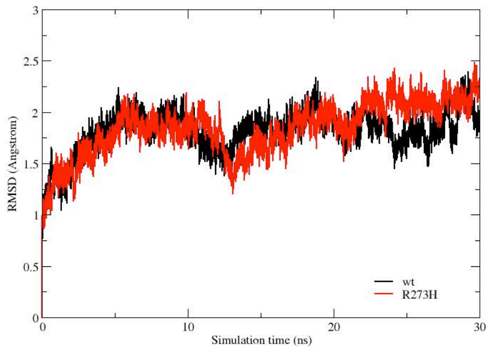
Figure S1. Root mean square deviations (RMSD) of C_{\alpha} atoms of p53 wild-type and mutant systems during simulations
