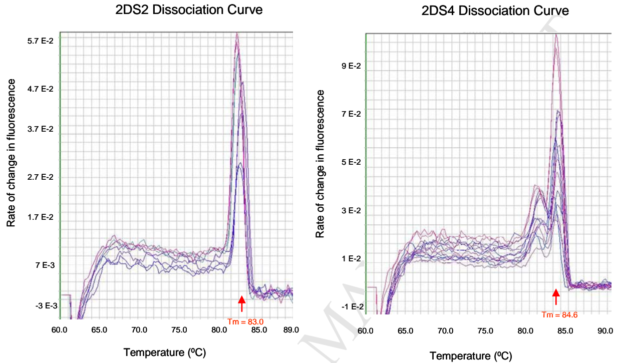
Supplement Figure 2. Dissociation curve for KIR2DS2 and KIR 2DS4 amplified products. All PCR products were reported only after assesement for the correct dissociation curve.
