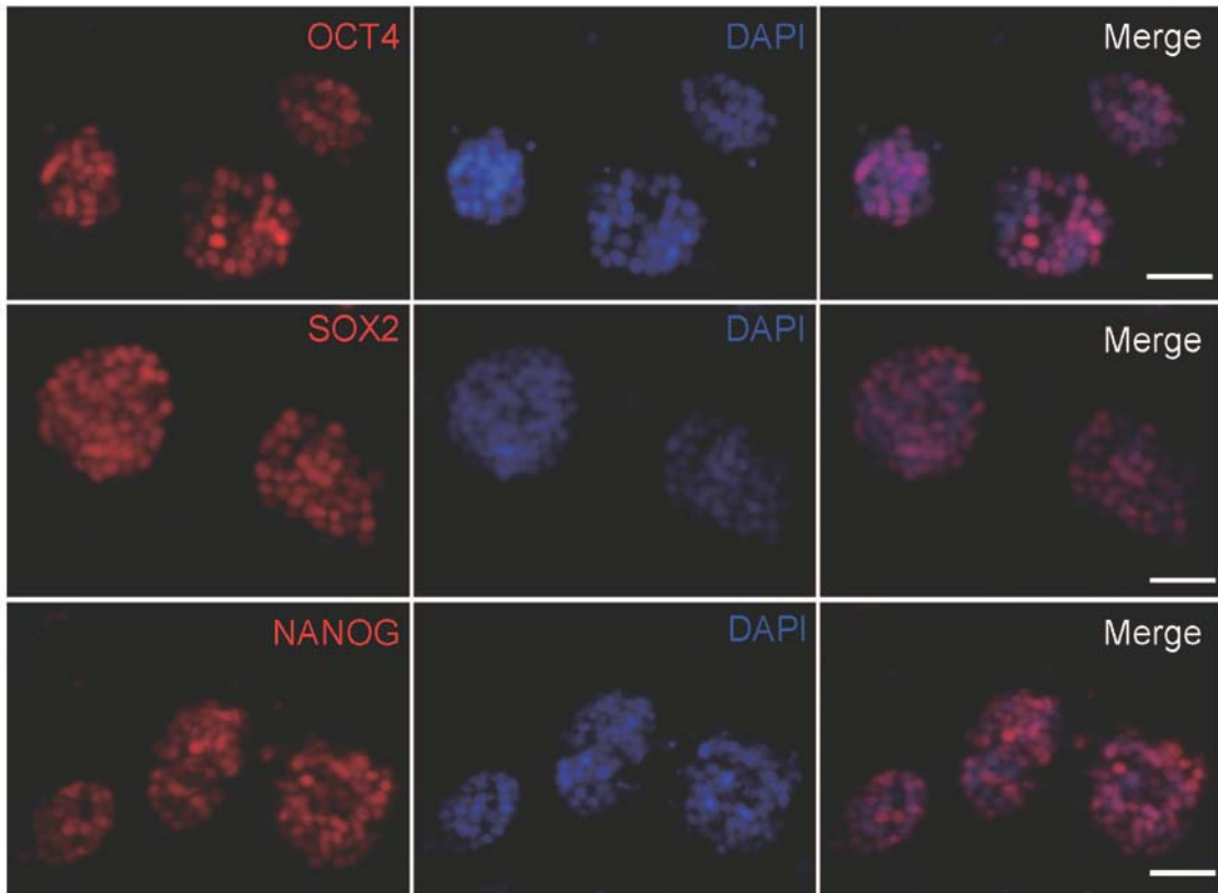
Figure S1 Immunostaining of OCT4, SOX2 and NANOG in sheep iPS cells. Scale bars: 50 μm.
