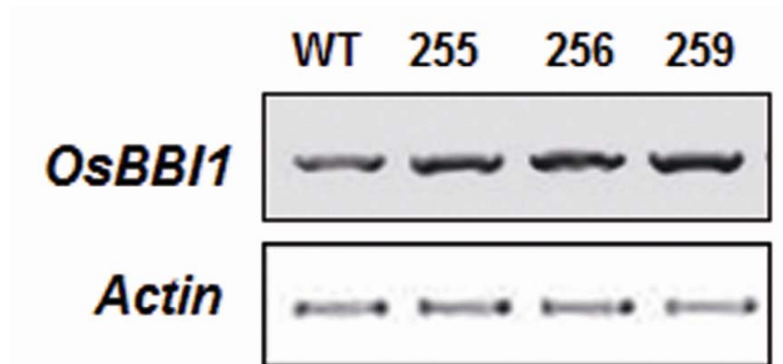
Supplementary information, Figure S3 Expression levels of OsBBI1 in transgenic lines.
