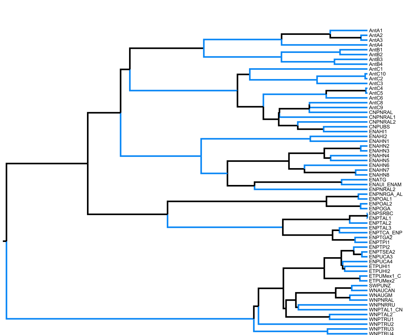
CYTB
