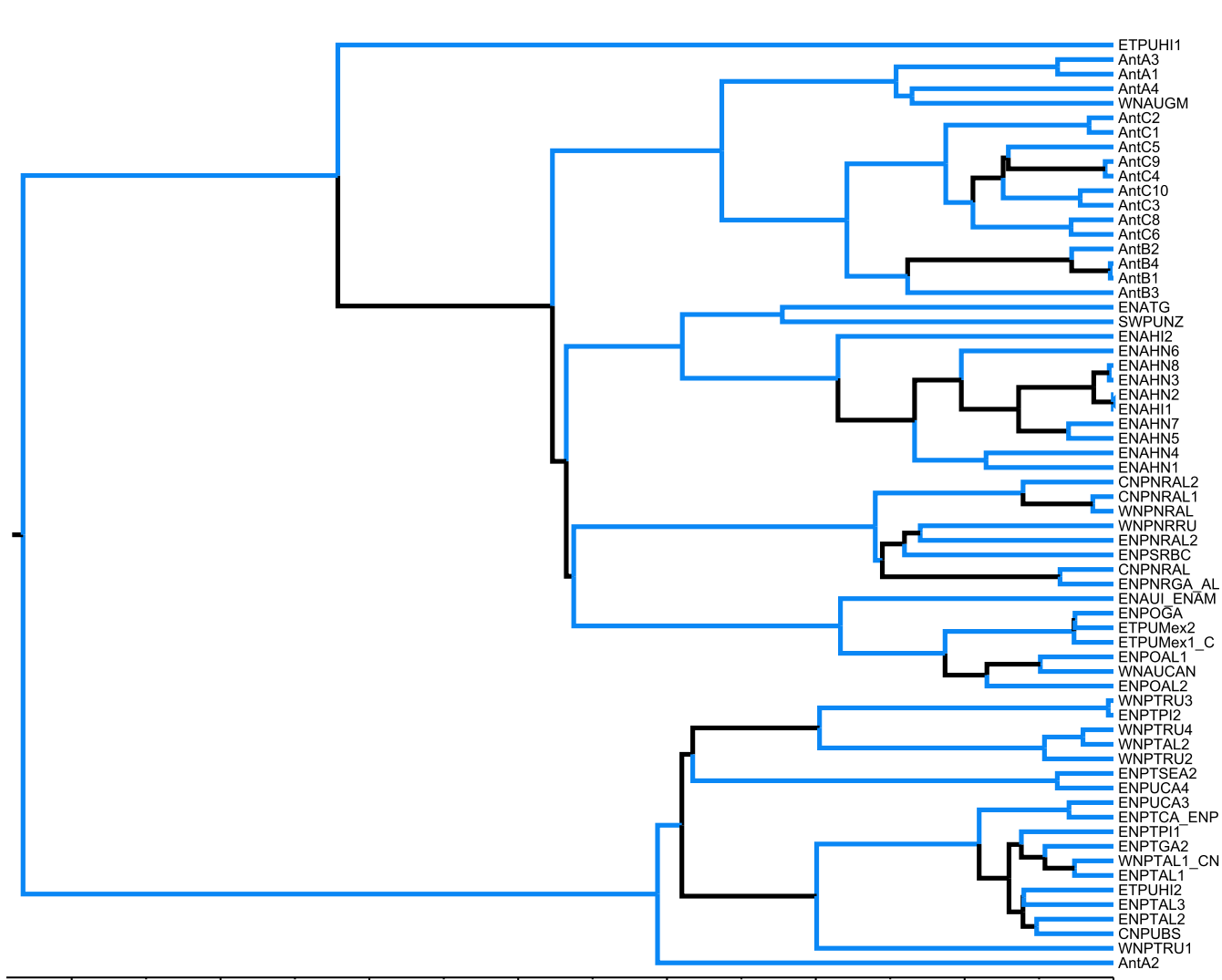
CR
