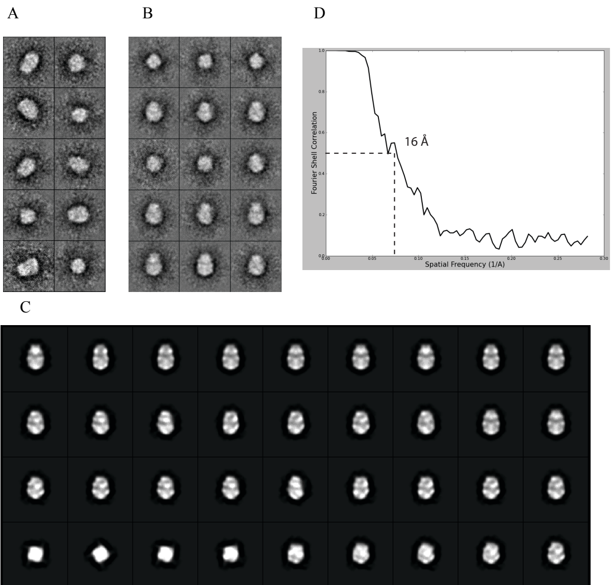
FIGURE S1. Single particle electron microscopy of TRPA1 in A8-35 amphiphol. A , Representative reference-free class average with no imposed symmetry. B , Four-fold symmetry imposed class averages. C , Back projections from the three-dimensional structure. D , Fourier shell correlation indicating a resolution of 16 Å (0.5 cutoff).
