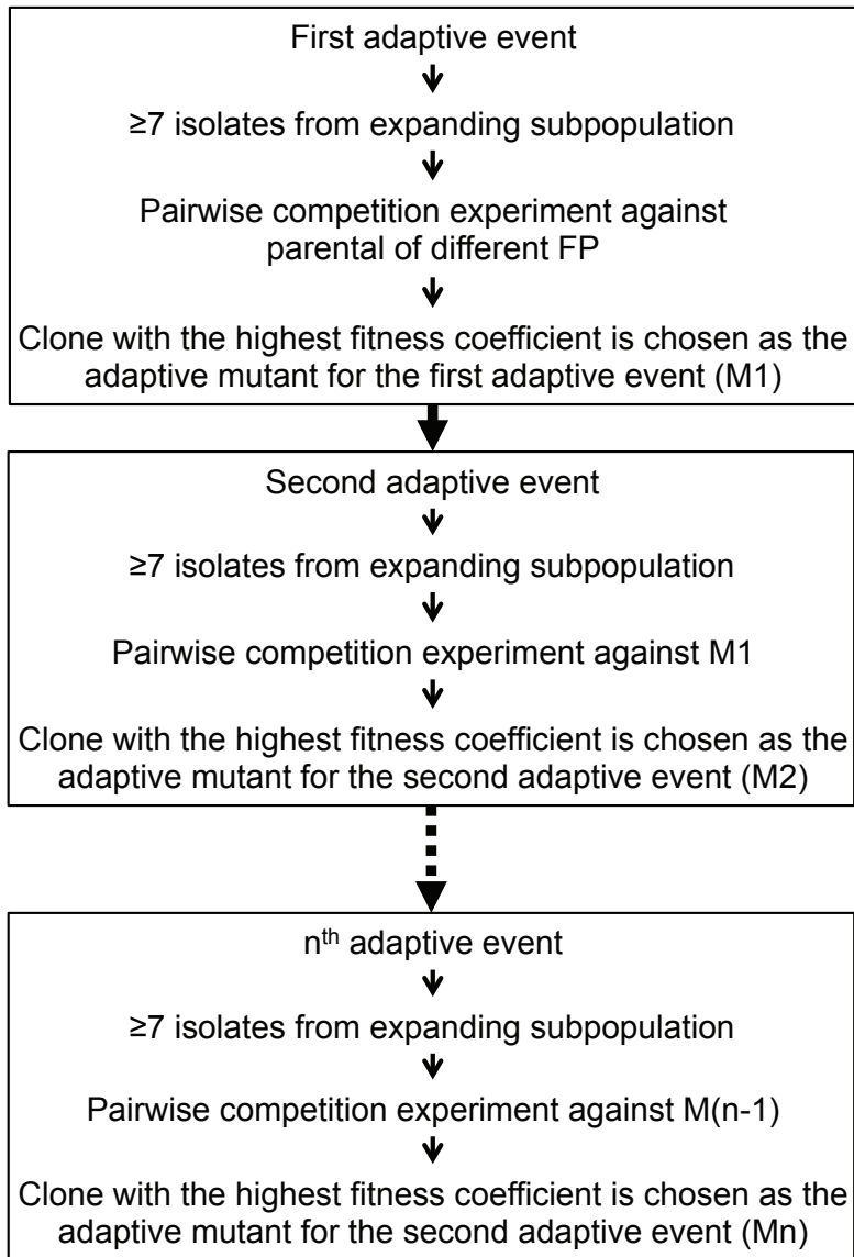
Figure S1. Process for identifying adaptive mutants. The pairwise competition experiments were performed in chemostats in the presence of the same concentration of fluconazole used during the evolution of these isolates.
