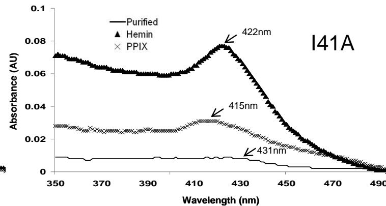
Figure S4: Spectra of absorbance (240-600nm, only 350-500 nm shown) of semi-purified WT and mutants in the absence or presence of 5 \mu M hemin and PPIX after heme reduction with 5mM DTT. UV-Vis was collected as described under Material and Methods.
