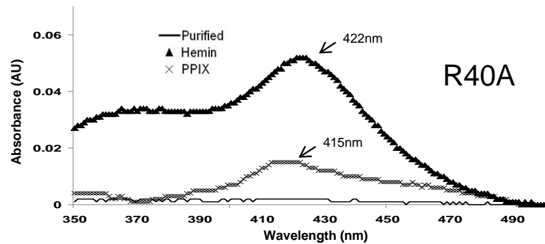
Figure S4: Spectra of absorbance (240-600nm, only 350-500 nm shown) of semi-purified WT and mutants in the absence or presence of 5 \mu M hemin and PPIX after heme reduction with 5mM DTT. UV-Vis was collected as described under Material and Methods.
