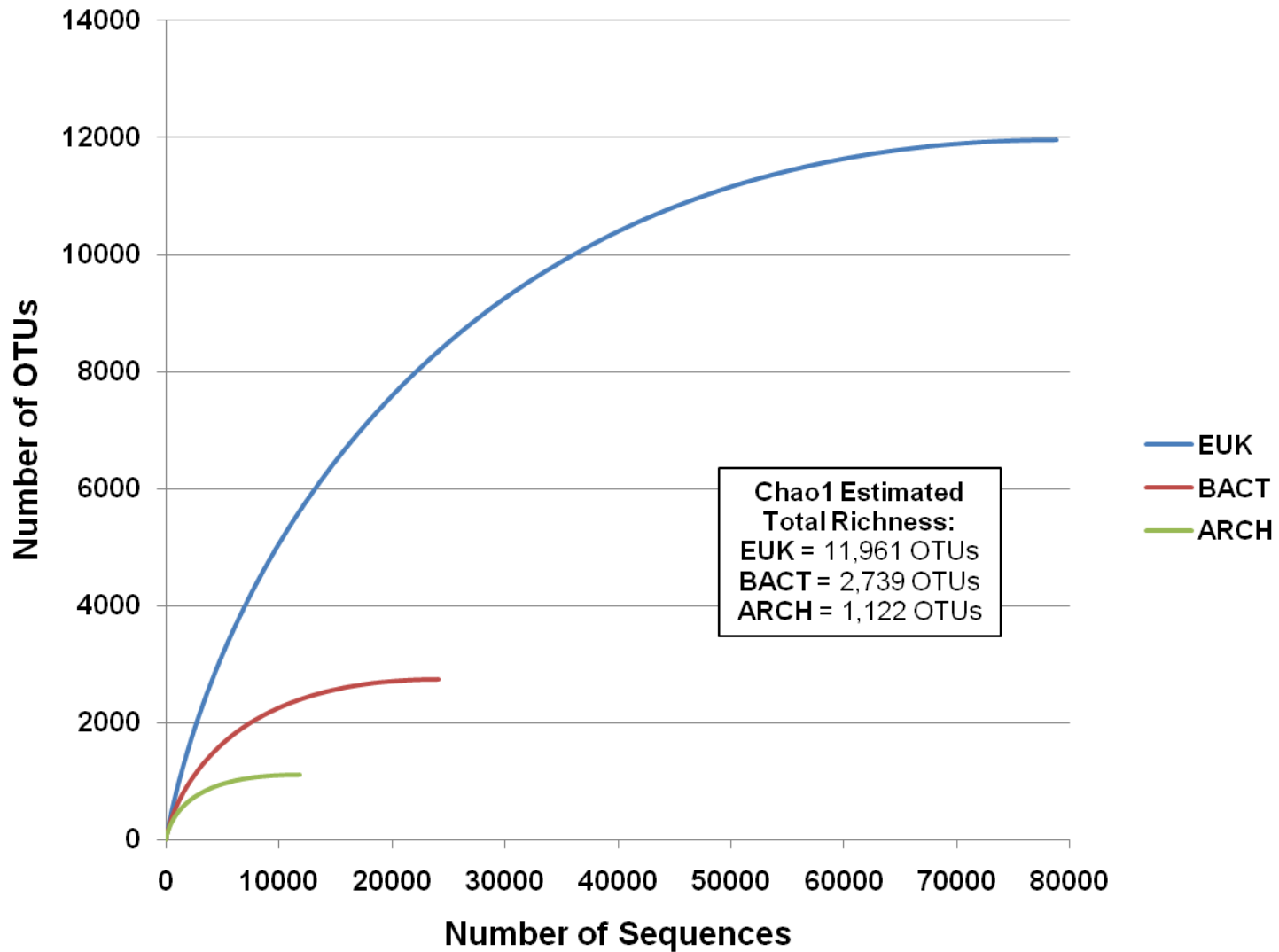
Figure S1. Rarefaction analysis for Bacteria (97% OTU level), Eukaryotes (98% OTU level) and Archaea (97% OTU level). The inset box shows the Chao1 total richness estimate for the three Domains.
