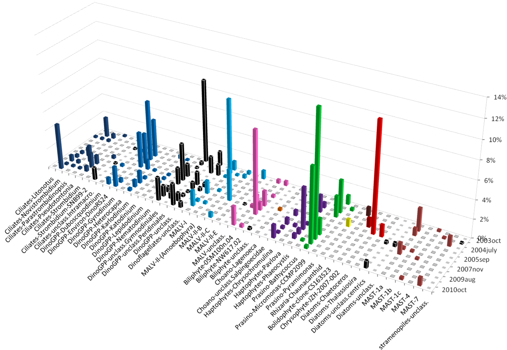
Figure S6. Taxonomic distribution of the top 50 dominant eukaryotic OTUs (98% level). Colors are as in Figure 4: the different sub-groups of Alveolates are in shades of blue, the Biliphytes in pink, the Choanoflagellates (Choano) in orange, the Haptophytes in purple, the Prasinophytes (Prasino) in green, the Rhizaria in yellow, the stramenopile sub-groups in shades of red and the unclassified (uncl.) levels in black. Intramacro., Intramacronucleata; DinoGPP, Gymnodinium-Peridinium-Prorocentrum complex; Environ, environmental; MALV, uncultured marine Alveolate group; MAST, uncultured marine stramenopile group. Gray squares indicate complete absence (0%).
