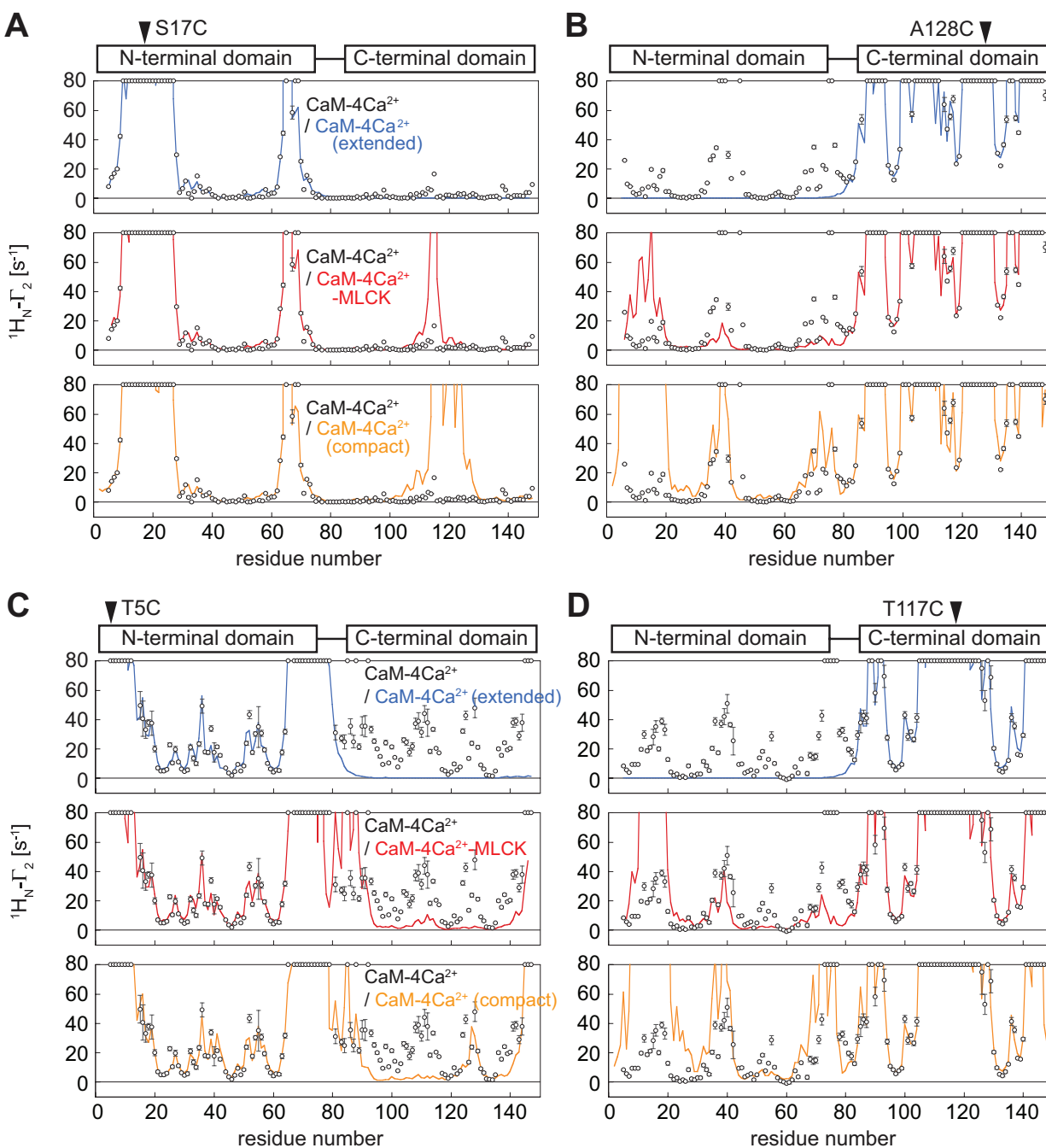
Fig. S4. PRE profiles for \text{Ca}^{2+} -loaded CaM. Experimental PRE profiles (circles, error bars = 1 s.d.) for \text{CaM-4Ca}^{2+} with the nitroxide spin label at (A) S17C, (B) A128C, (C) T5C, and (D) T117C. Where the PRE is too large to be accurately measured ( \geq 80 \text{ s}^{-1} ), the experimental PREs are plotted at the top. PRE profiles back-calculated from known structures are shown as solid lines: \text{CaM-4Ca}^{2+} in the dumbbell conformation (blue, PDB 1CLL S5 ), \text{CaM-4Ca}^{2+} -MLCK (red, PDB 1CDL S3 ), and \text{CaM-4Ca}^{2+} in the compact conformation (orange, PDB 1PRW S6 ). Paramagnetic tag conformations, represented by a five-member ensemble, were first obtained by fitting the intradomain PREs only; these positions were then used to back-calculate the PRE profiles for the rest of the protein. Note that panels C and D show raw PRE profiles (see Fig. S5).
