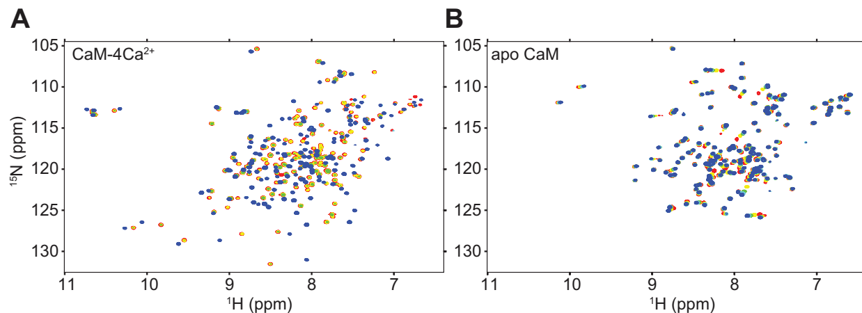
Fig. S2. ^1\text{H}_\text{N}/^{15}\text{N} chemical shift perturbations in CaM upon binding MLCK CBD peptide. (A) ^1\text{H}-^{15}\text{N} HSQC spectra of ^{15}\text{N} -labeled \text{Ca}^{2+} -loaded CaM (100 \mu\text{M} ) with 0 (red), 0.33 (yellow), 0.67 (green), 1 (cyan), and 1.2 (blue) equivalents of unlabeled MLCK peptide. (B) ^1\text{H}-^{15}\text{N} HSQC spectra of ^{15}\text{N} -labeled apo CaM (100 \mu\text{M} ) with 0 (red), 0.5 (yellow), 1 (green), 1.5 (cyan), and 2 (blue) equivalents of unlabeled MLCK peptide. The interaction between \text{Ca}^{2+} -loaded CaM and MLCK peptide is slow on the chemical shift time scale (i.e. two sets of cross-peaks are observed for unbound and peptide-bound CaM), whereas that with apo CaM is fast on the chemical shift time scale (i.e. a single set of cross-peaks with shifts at the weighted average of unbound and peptide-bound apo CaM). The slower timescale of the interaction for \text{Ca}^{2+} -loaded CaM and the greater magnitude of the chemical shift perturbations upon peptide binding (Fig. 1D main text), which are seen throughout the protein, are indicative of a larger binding interface and major structural rearrangements upon binding, consistent with the formation of the compact structure determined by NMR S2 and crystallography. S3 The much faster exchange kinetics and smaller chemical shift perturbations seen for apo CaM indicate that little structural change occurs upon peptide binding. That these perturbations are largely localized to the C-terminal domain indicates that the peptide only interacts primarily with the C-terminal domain and does not induce interdomain closing of apo CaM.
