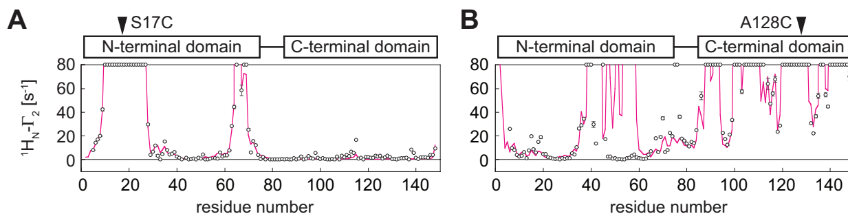
Fig. S7. Comparison of experimental PREs for \text{Ca}^{2+} -loaded CaM with those calculated from a molecular dynamics simulation. The experimental PRE profiles (open circles) are presented as in Fig. 2 of the main text; PREs back-calculated from a published molecular dynamics (MD) ensemble (PDB 2K0E S9 ) are displayed as magenta lines. Paramagnetic tag conformations, represented by a five-member ensemble, were obtained by fitting the intradomain PREs only, and these positions were then used to back-calculate the PRE profiles for the remainder of the protein. The MD ensemble (which consists of 160 structures) predicts some, but not all, features of the experimental interdomain PRE profiles. The MD ensemble was generated using a complete empirical energy force field, in conjunction with restraints for intradomain NOEs and relaxation-derived backbone amide order ( S^2 ) parameters; S9 thus there are no interdomain experimental restraints to drive the relative positioning of the two domains. The MD simulations show that the N- and C-terminal domains of CaM-4Ca ^{2+} can potentially sample a wide range of relative orientations, including some similar to the peptide-bound state, although not in any preferential manner as demonstrated by the experimental PRE data. The MD simulations also predict additional close-contact structures that are not compatible with the PRE data (particularly apparent for residues 47-59 in the A128C PRE data set shown in panel B and misses others (e.g. residues 138 and 139 in panel A and 15-19 in panel B ).
