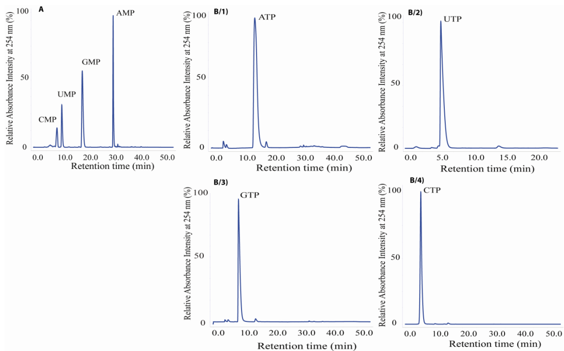
Figure S1. Reverse phase FPLC chromatograms of the separation of ribonucleoside monophosphates (NMPs) and enzymatic phosphorylation of labeled NMP to NTP. (A) NMP mixtures were separated on a Targa C18 reverse phase column ( 250 \times 4.6 mm, 5 \mu\text{m} , Higgins Analytical, Inc.) at a flow-rate of 0.8 ml/min using solvent A ( 0.1 \text{ M KH}_2\text{PO}_4 ) and B ( 20\% \text{ v/v MeCN} in 0.1 \text{ M KH}_2\text{PO}_4 ) with detection at 254 nm. (B) Enzymatic phosphorylation of labeled NMP to NTP is complete after 1 hr (same FPLC condition as (A) ).
