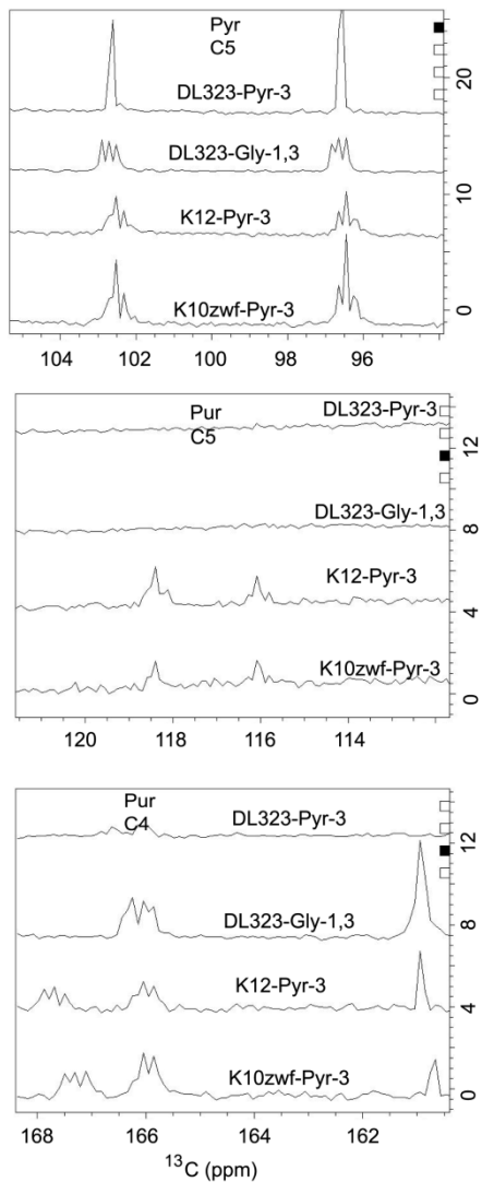
Figure S2. Labeling pattern of a mixture of four rNMPs isolated from K10zwf , K12 , and DL323 E. coli grown in a [3-^{13}\text{C}] -Pyruvate background, and DL323 E. coli grown in a [1, 3-^{13}\text{C}] -glycerol background. The direct carbon detection 1D spectrum shows all the labeled carbon positions. A long recycle delay of 5 s was used to allow for sufficient magnetization recovery and proton decoupling was limited to the acquisition period only. The residual ^{13}\text{C} - ^{13}\text{C} coupling observed in a [1, 3-^{13}\text{C}] -glycerol is absent with the [3-^{13}\text{C}] -Pyruvate only in DL323 ; K10zwf and K12 grown in [3-^{13}\text{C}] -Pyruvate still retain the residual ^{13}\text{C} - ^{13}\text{C} coupling.
