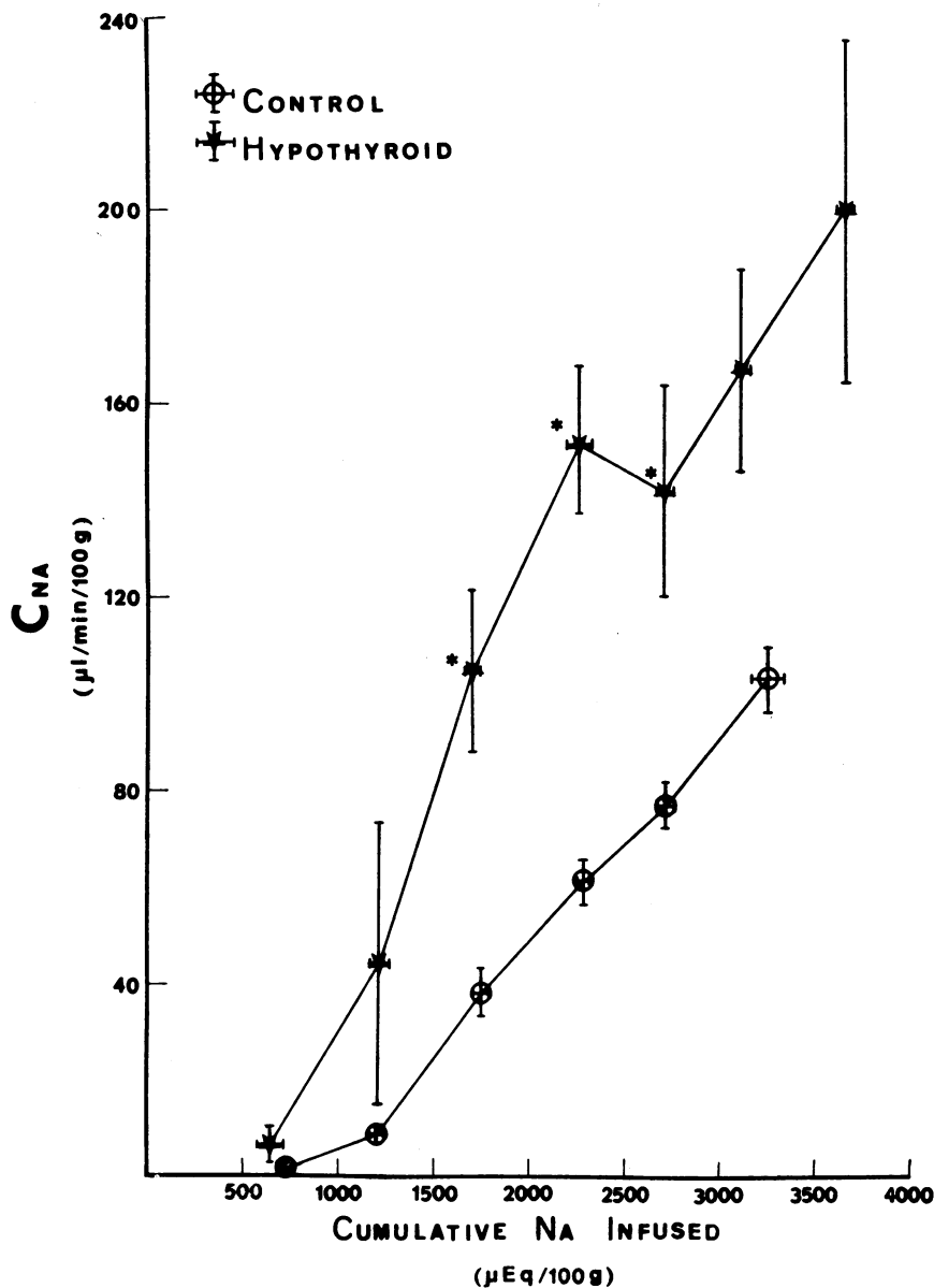
FIGURE 1 Sodium clearance in nine hypothyroid and seven control rats. The mean C_{Na} \pm \text{SEM} for each increment of 500 \mu\text{Eq} of infused sodium is plotted against the mean cumulative sodium infused \pm \text{SEM} for this same increment. * indicates those means of the C_{Na} which are significantly different ( P < 0.05 or less) when hypothyroid and control values are compared.
