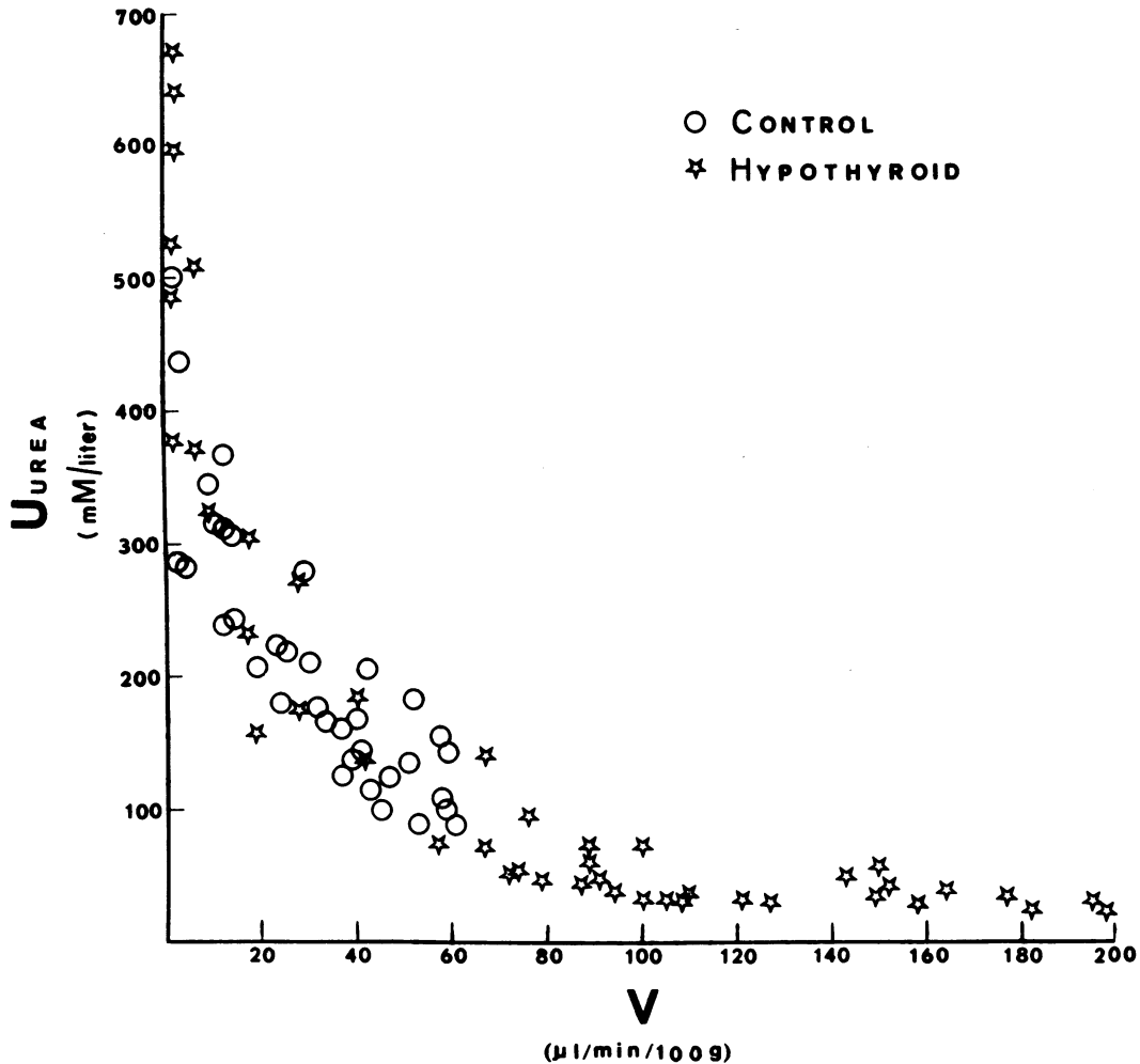
FIGURE 7 Urinary urea concentration relative to urine flow rate. Values for U_{\text{urea}} and V represent data obtained during the equilibration period and throughout the saline diuresis.
