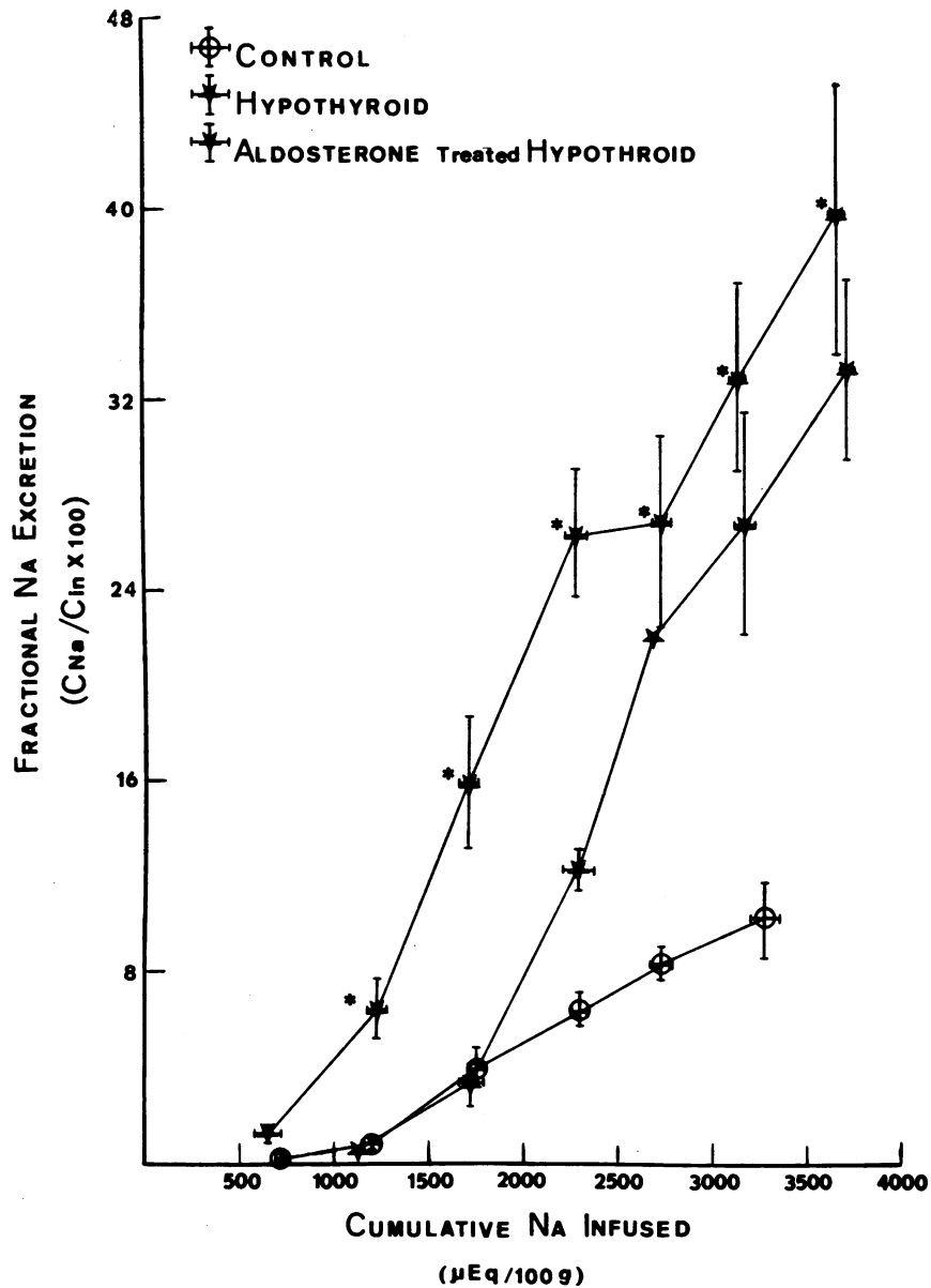
FIGURE 2 Fractional sodium excretion in nine hypothyroid and seven control rats. The mean fractional sodium excretion \pm SEM for each increment of 500 \mu Eq of infused sodium is plotted against the mean cumulative sodium infused \pm SEM for this same increment. The three curves represent three different groups of rats: untreated control, untreated hypothyroid, and aldosterone-treated hypothyroid. * indicates those means of the fractional sodium excretion which are significantly different ( P < 0.02 or less) when untreated hypothyroid and control values are compared.
