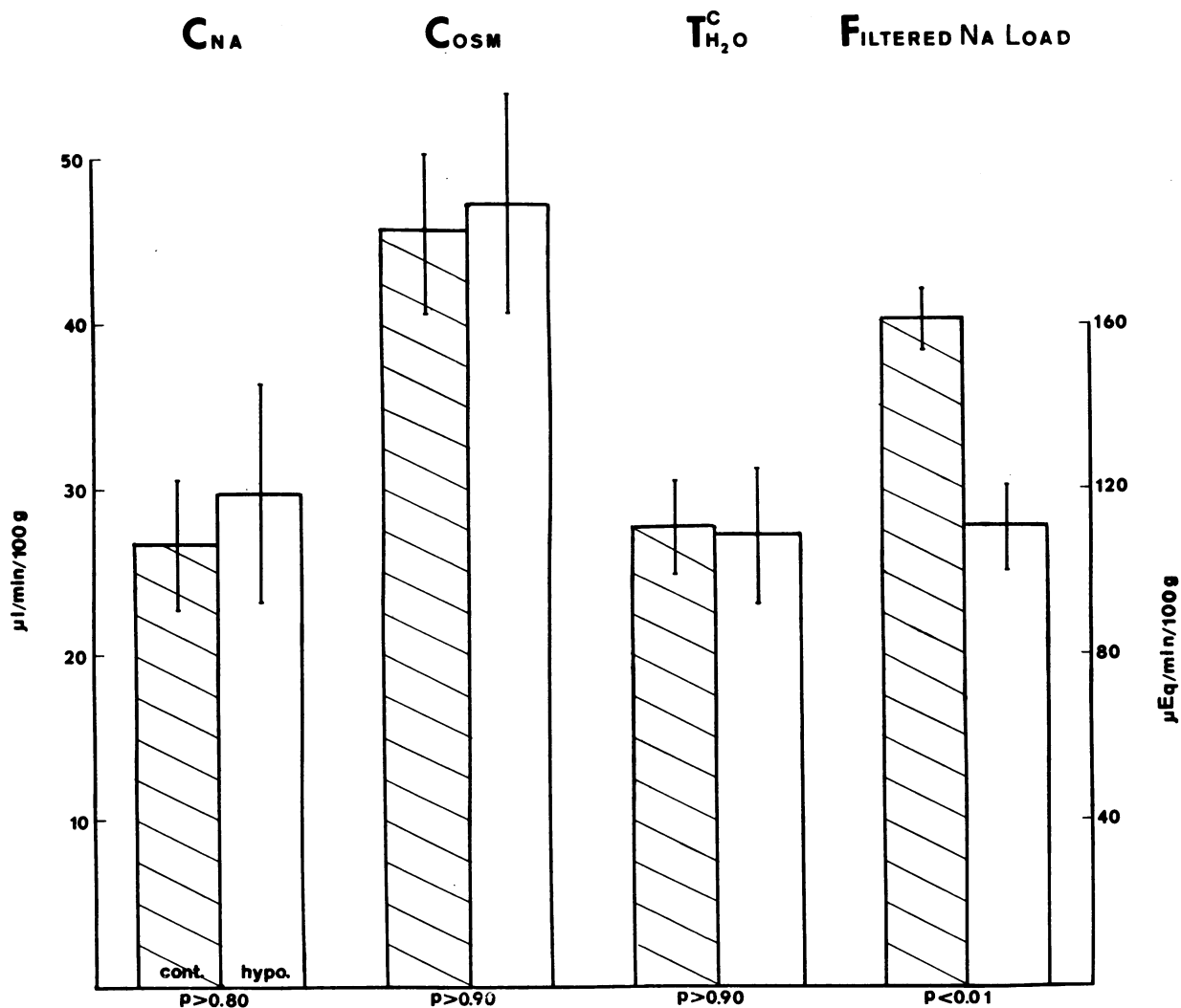
FIGURE 5 Comparison of C_{Na} , C_{Osm} , T_{H_2O}^c , and filtered sodium load in control (cont.) and hypothyroid (hypo.) rats when the C_{Osm} was less than 90 \mu\text{l}/\text{min} per 100\text{ g} . Each bar in the controls, 30 observations, and each bar in the hypothyroids, 13 observations, represents the mean \pm SEM for all clearance periods in each group over this C_{Osm} range.
