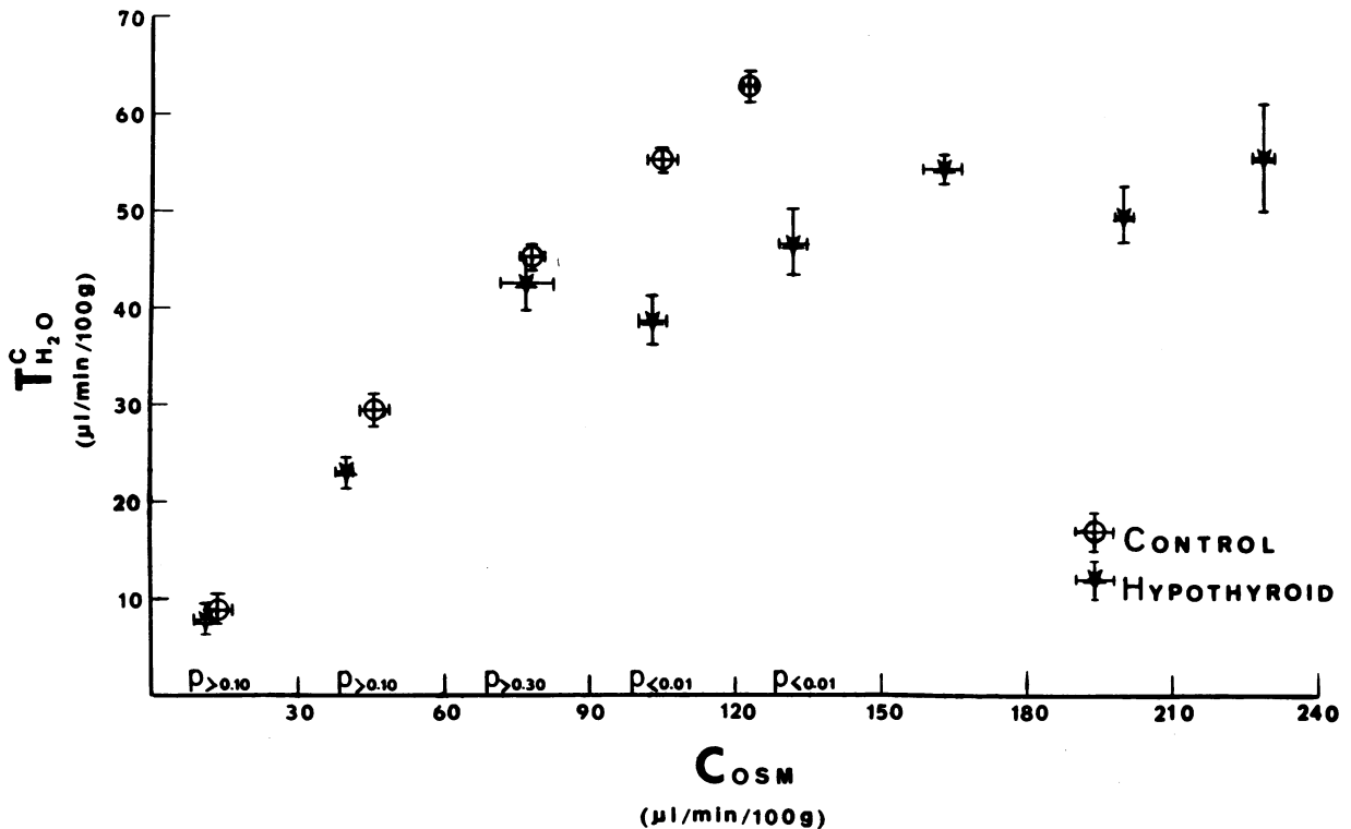
FIGURE 3 Solute free water reabsorption in hypothyroid and control rats. The means ± SEM for T c H 2 O and C osm were computed for both groups for each C osm increment of 30 μl. The mean T c H 2 O per C osm was compared in hypothyroid and control rats in each increment of C osm and the P value is recorded on the abscissa.
