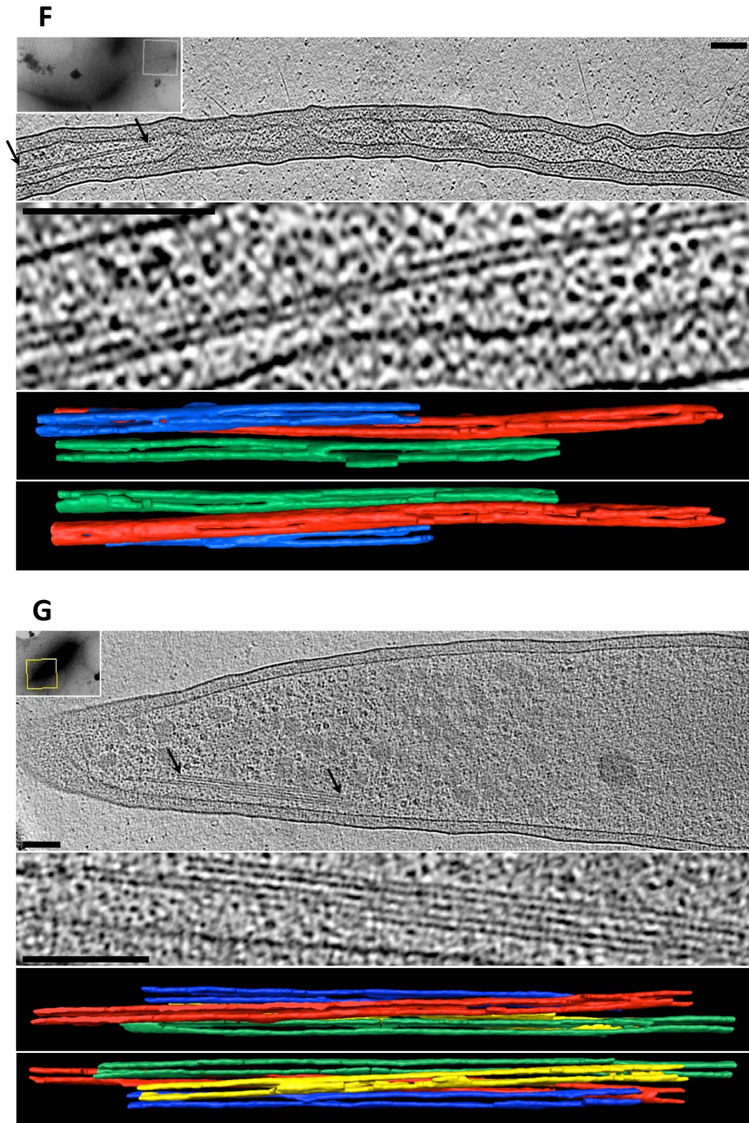
Figure S3. Additional examples of bacterial microtubules in Prosthecobacter .
