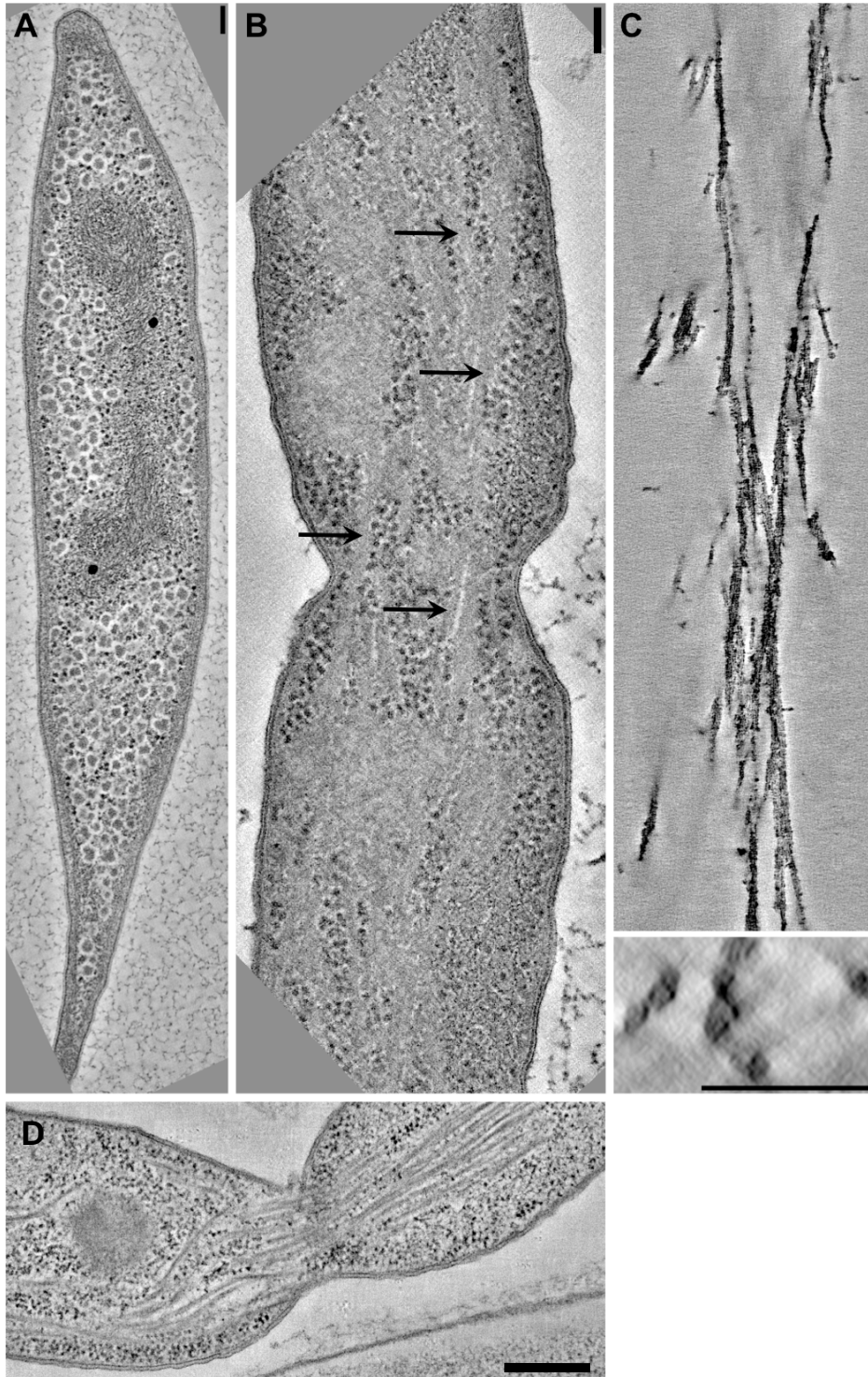
Figure S4. BtubA/B-structures are not preserved well by conventional EM methods.
