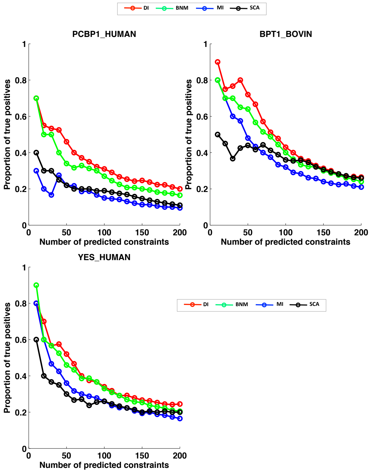
Figure S6. True positive rate of predicted contacts for 4 methods
