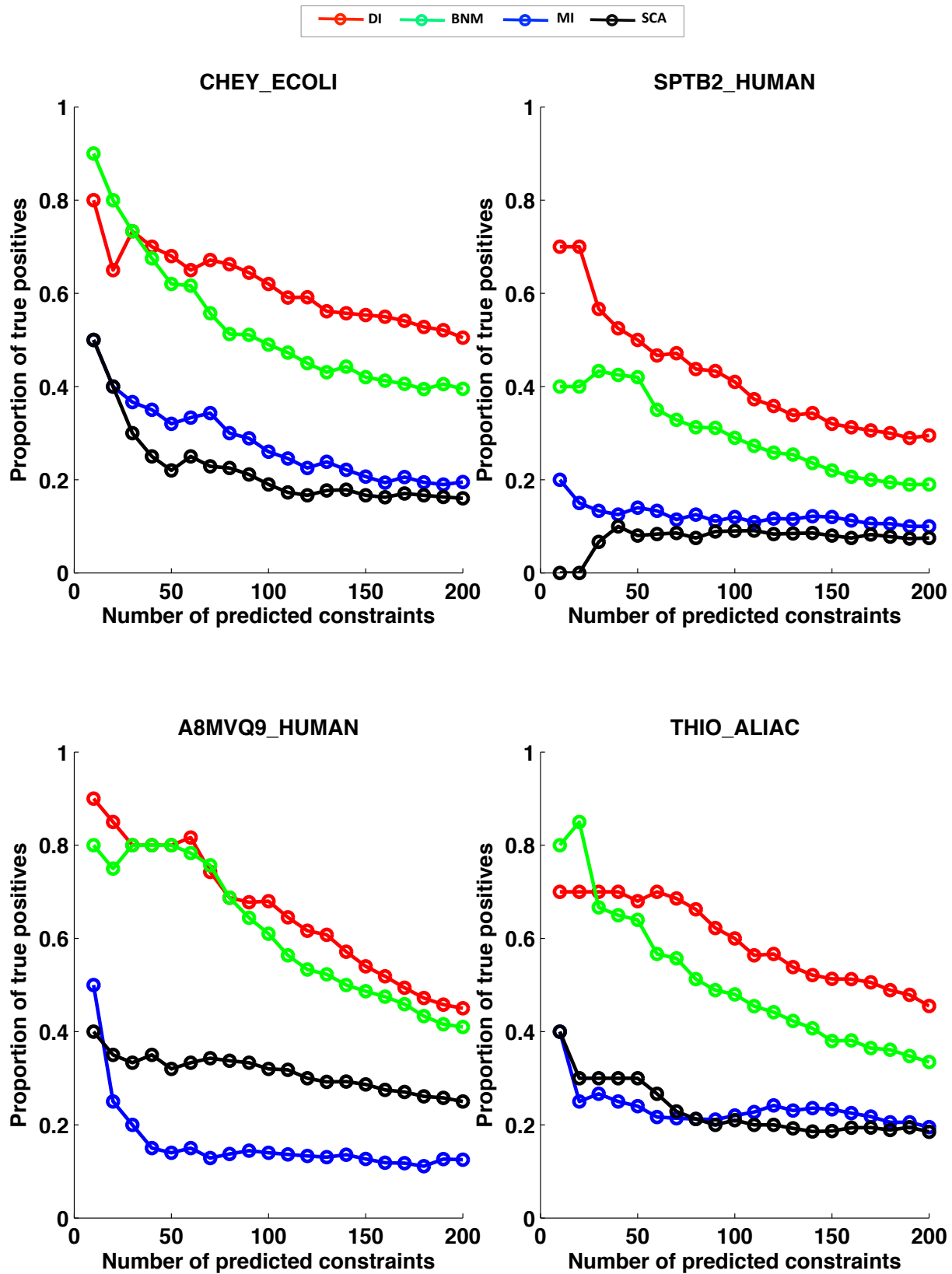
Figure S6. True positive rate of predicted contacts for 4 methods
