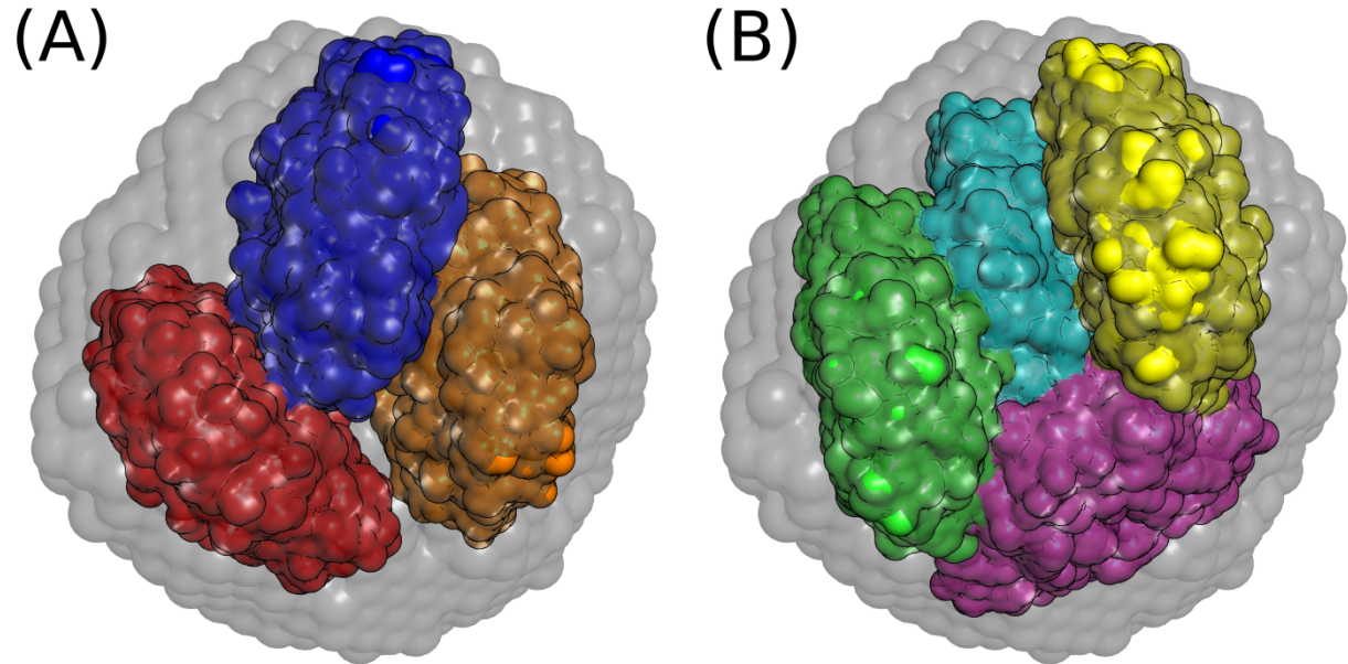
Supplemental Figure 1S. A superposition of the average bead model envelope for rsAra h 1 with the rigid body models for three (A) and four (B) trimeric assemblies, respectively. The average bead model envelope was constructed with DAMAVER. The rigid body models depict possible arrangements of the oligomeric states computed with SASREF. The alignment was conducted using SUPCOMB.
