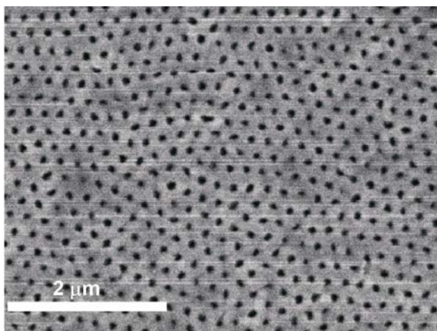
Supporting Information Figure 1: SEM image of anodic alumina oxide template with 85 nm diameter pore.
