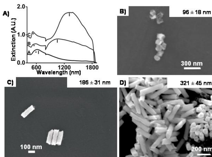
Supporting Information Figure 2: A) UV-vis-NIR spectra for: 96 nm (bottom), 186 nm (middle), and 321 nm (top) long gold rods. SEM images of: B) 96 nm, C) 186 nm, and D) 321 nm long gold rods.
