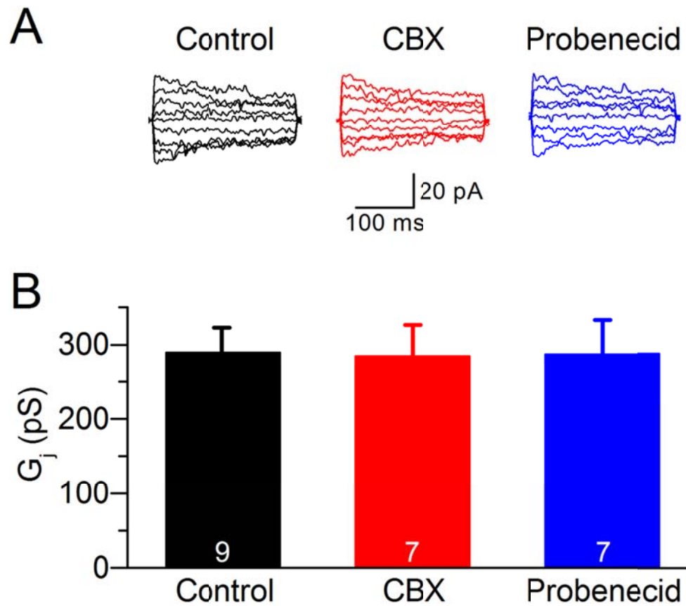
Supplementary Figure 1. Neither carbenoxolone (CBX) nor probenecid inhibited electrical coupling of C. elegans body-wall muscle. A , Sample junctional current traces from control cells and cells treated with either CBX (50 \mu M) or probenecid (100 \mu M). B , Comparisons of junctional conductance ( G_j ) among the different groups. Shown are mean \pm SE. Data are shown as mean \pm SE. There was no significant difference among the different treatment groups.
