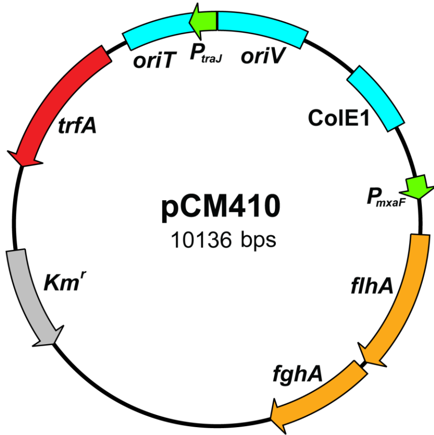
Figure S6. The physical map of the pCM410 plasmid (GenBank accession no. FJ389188). P mxaf , strong, endogenous methanol dehydrogenase promoter; flhA and fghA , enzymes of the introduced GSH dependent formaldehyde oxidation pathway; trfA , plasmid replication initiator gene; oriV , IncP origin of replication; oriT , origin of transfer; colE1 , high-copy origin of replication in E. coli ; Km r , kanamycin resistance marker.
