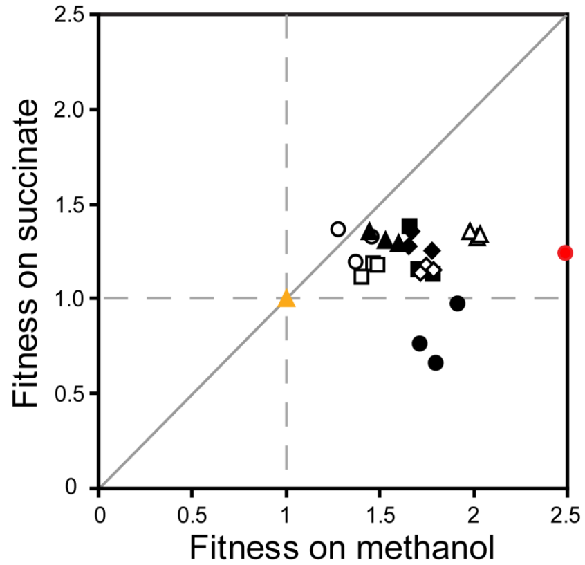
Figure S4. Fitness on methanol vs. succinate. WT, red circle; EM, orange triangle; three evolved isolates from each of F1 through F8 after 600 generations in methanol (●, ○, ▲, △, ■, □, ◆, ◇).
