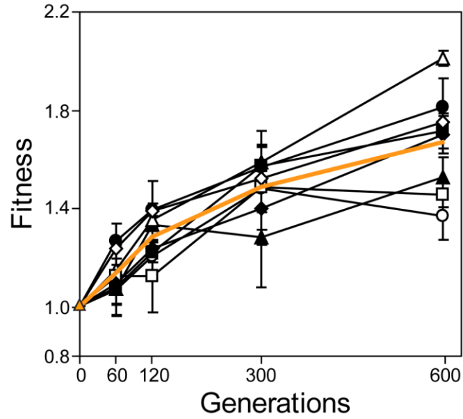
Figure S3. Dynamics of adaptation of the EM strain evolved in medium containing methanol. Fitness increases through time for replicate populations F1 through F8 (●, ○, ▲, △, ■, □, ◆, ◇). Orange triangles and line indicate the EM strain and the grand population mean, respectively.
