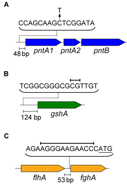
Figure S5. Three focal mutations related to C_1 metabolism. Details of the genetic changes and relationship to methylotrophy in the EM strain are discussed above in Supplemental Text.
