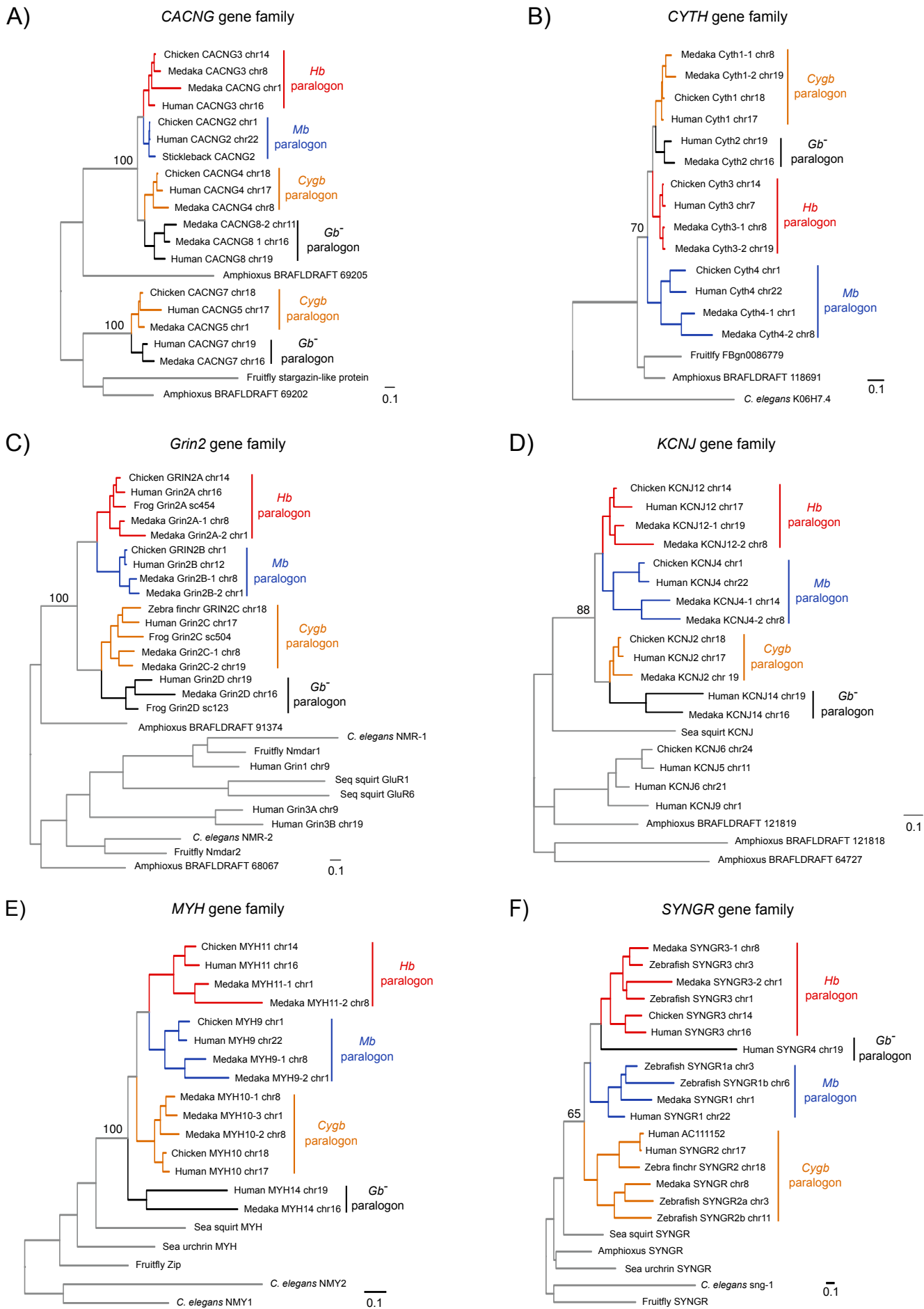
Supplementary figure 3. Maximum likelihood phylogenies of six vertebrate gene families that unite the three globin-defined paralogs with the Gb - paralogon, located on human chromosome 19. In each case the gene families diversified prior to the divergence of tetrapods and teleost fish. Numbers above the nodes correspond to maximum likelihood bootstrap support values.
