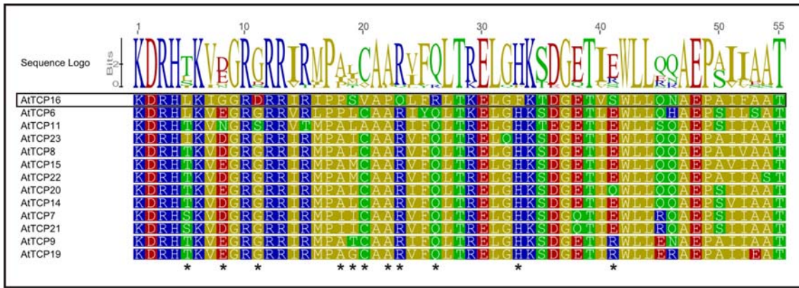
Supplemental Fig. 1. TCP domain sequences of Arabidopsis class I TCP proteins. The sequence of TCP16 is boxed. Basic, acid, hydrophobic and hydrophilic residues are marked with different colors. In the upper part, the derived consensus sequence is shown in a sequence logo. Positions not conserved in TCP16 are marked with an asterisk.
